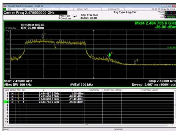
,Plot 2,Band Edge-802.11n(HT40) ,2452MHz,Ant1
