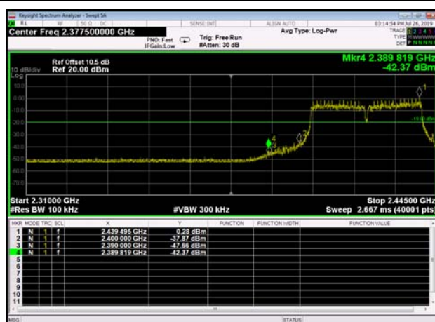
,Plot 2,Band Edge-802.11n(HT40) ,2437MHz,Ant1
