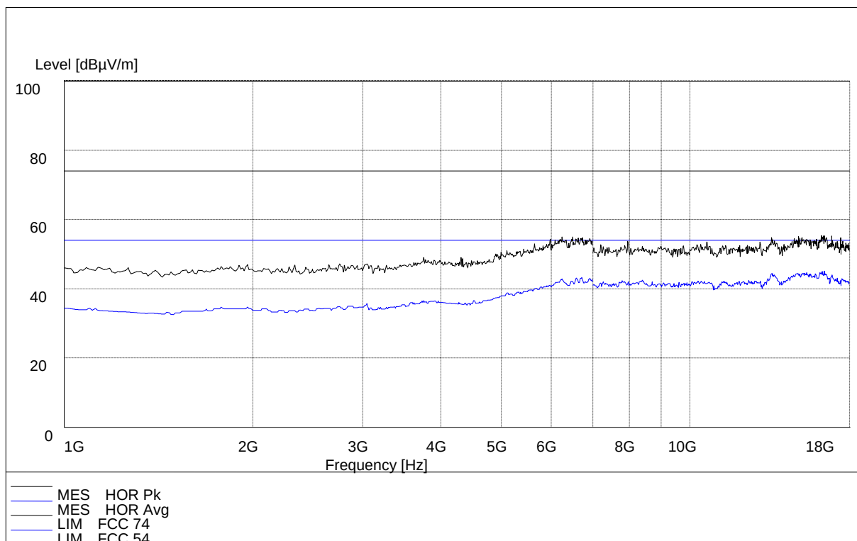
(Plot E: Test Antenna Horizontal 1G – 18G)
