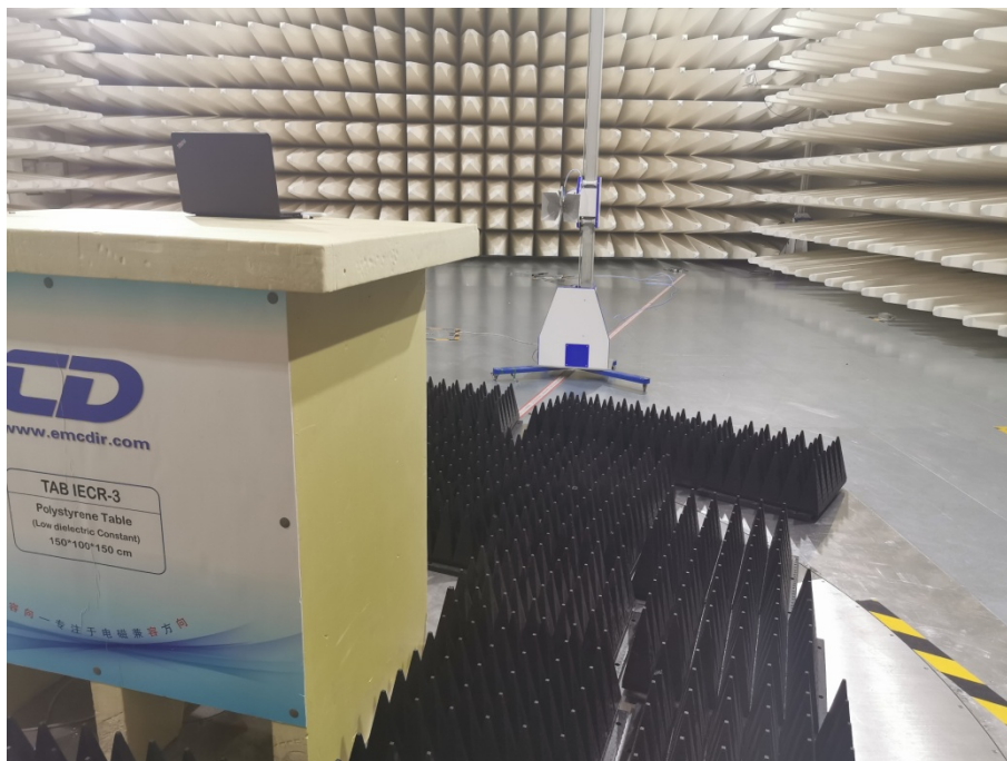
Spurious Radiated Emissions Test setup (Above 1GHz)
