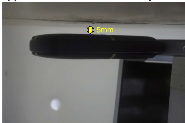
Direct Laptop Plug-in for USB Configuration 1 (Horizontal Up, Test Separation 5 mm)
