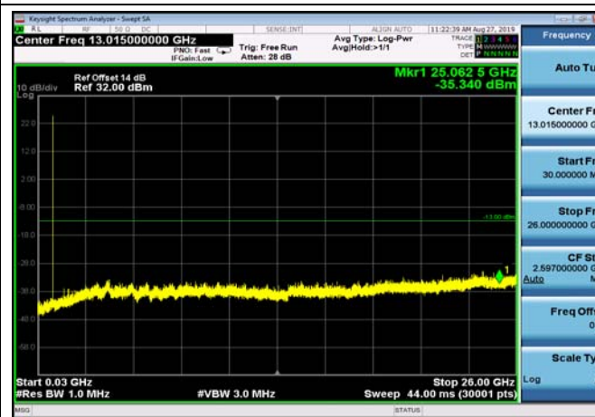
FDD05_LowRange_3MHz_30MHz~26GHz
