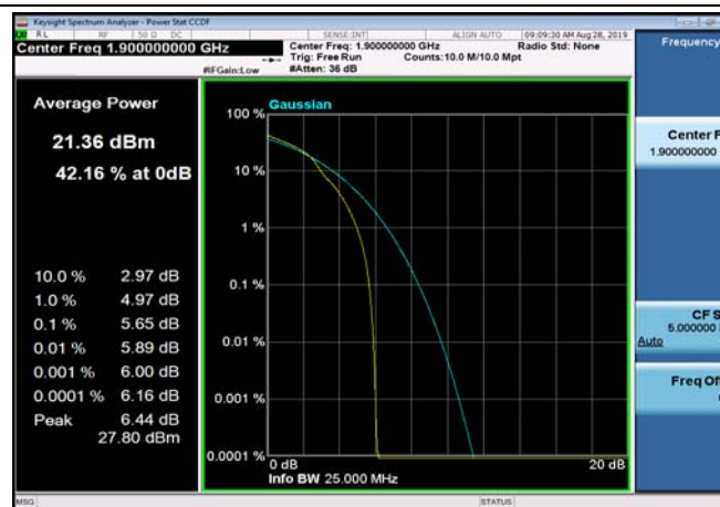
FDD02_HighRange_20MHz_1900_OneRB _high_Q16
