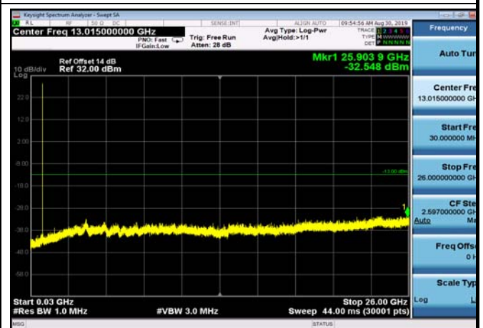
FDD05_LowRange_1.4MHz_30MHz~26GHz
