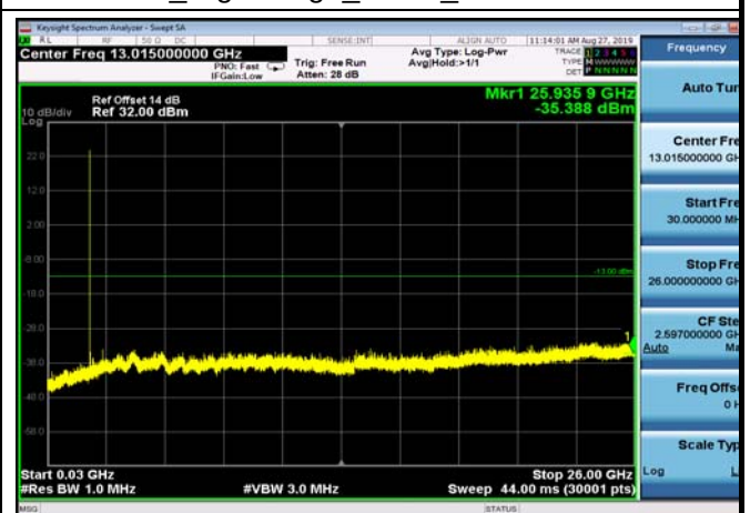
FDD02_HighRange_3MHz_30MHz~26GHz
