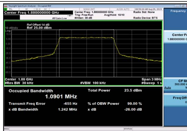
FDD02_MidRange_3_1880_QPSK
