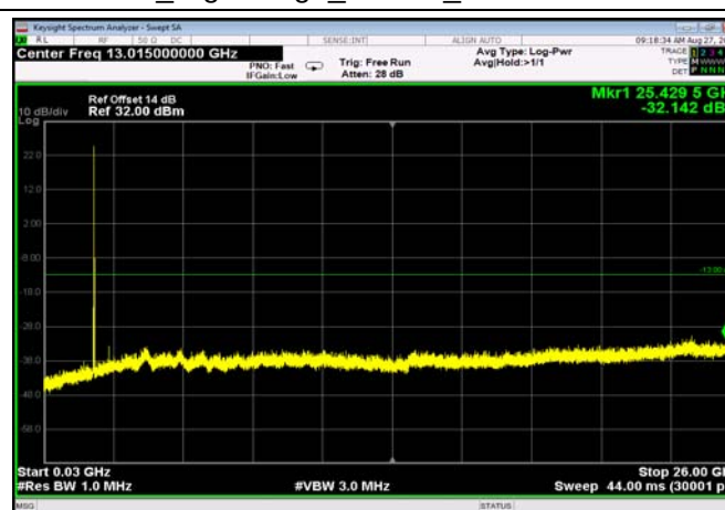
FDD02_HighRange_20MHz_30MHz~26GHz
