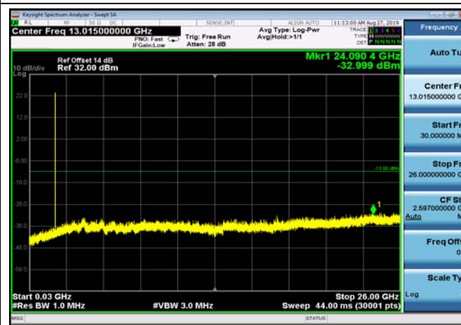
FDD02_MidRange_10MHz_30MHz~26GHz
