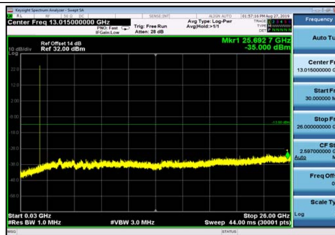
FDD02_HighRange_10MHz_30MHz~26GHz
