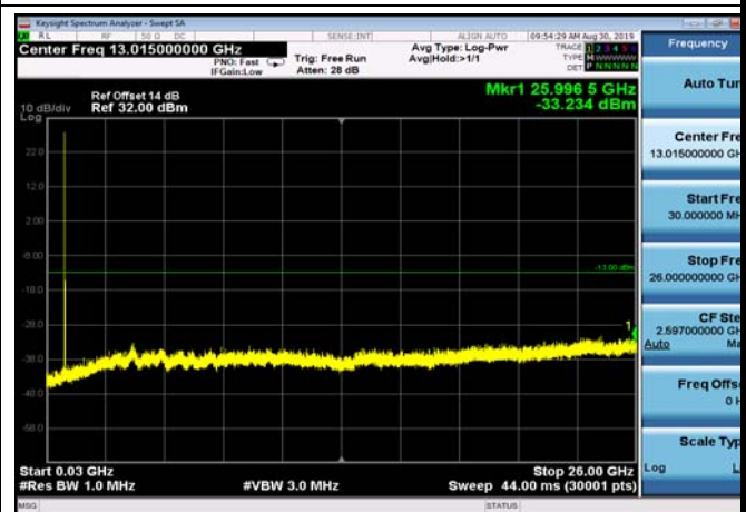
FDD07_LowRange_20MHz_30MHz~26GHz
