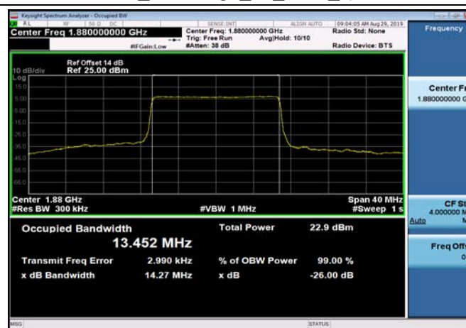
FDD02_MidRange_20_1880_QPSK
