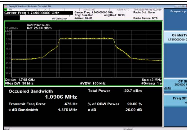
FDD66_MidRange_1.4MHz_1745MHz_QPSK
