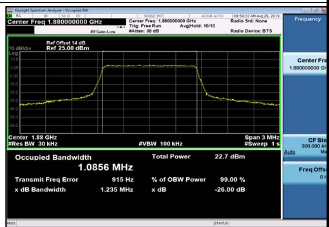
FDD02_MidRange_3_1880_Q16
