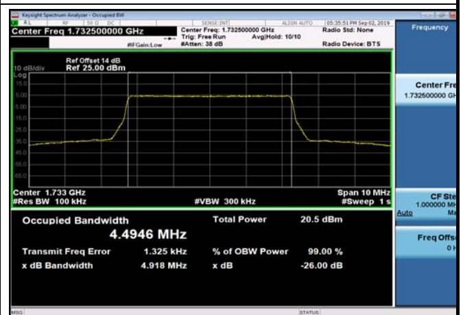
FDD04_MidRange_10_1732.5_Q16
