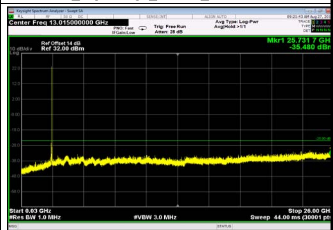
FDD07_HighRange_15MHz_30MHz~26GHz
