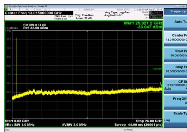
FDD07_HighRange_10MHz_30MHz~26GHz
