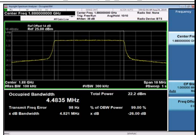
FDD02_MidRange_5_1880_Q16
