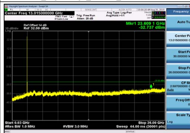
FDD07_HighRange_10MHz_30MHz~26GHz
