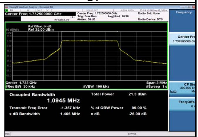
FDD04_MidRange_1.4MHz_1732.5MHz_Q16
