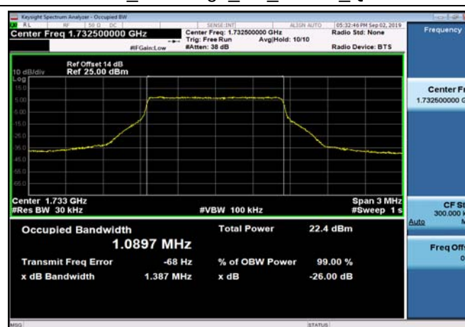
FDD04_MidRange_1.4_1732.5_QPSK
