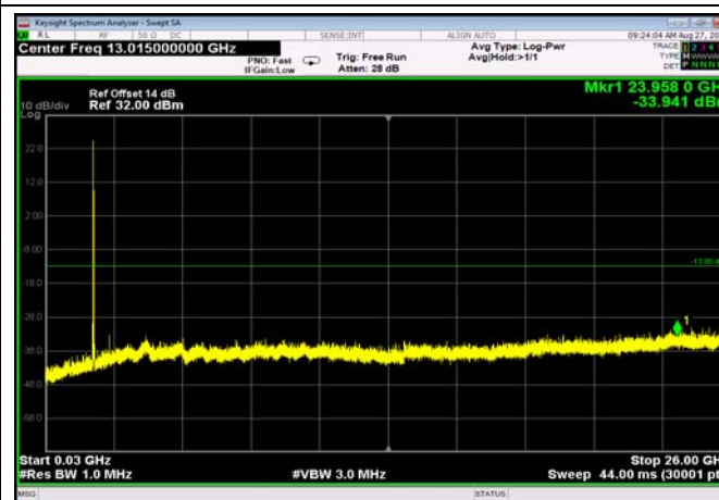
FDD02_LowRange_10MHz_30MHz~26GHz
