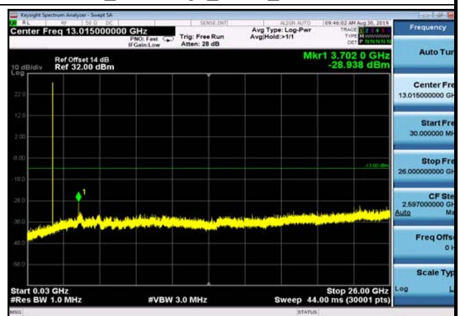
FDD02_MidRange_1.4MHz_30MHz~26GHz
