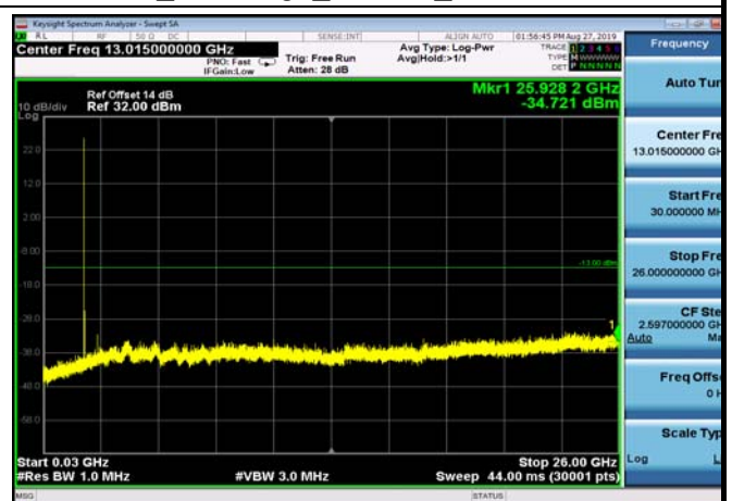
FDD02_MidRange_1.4MHz_30MHz~26GHz
