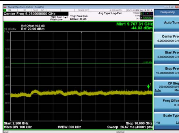
,Plot 4,2500MHz~10000MHz-802.11g ,2462MHz,Ant1
