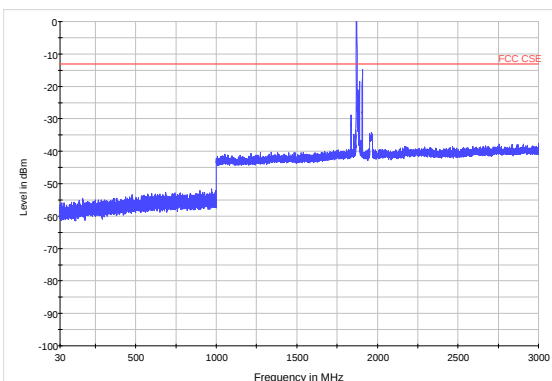
LTE Band 2 20MHz CH-Middle 30MHz~3GHz
