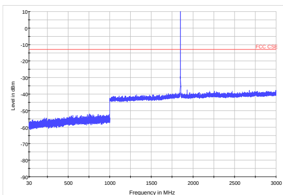
LTE Band 2 1.4MHz CH-Low 30MHz~3GHz
