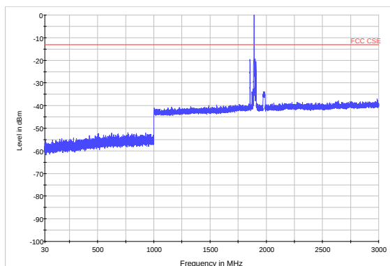
LTE Band 2 20MHz CH-High 30MHz~3GHz
