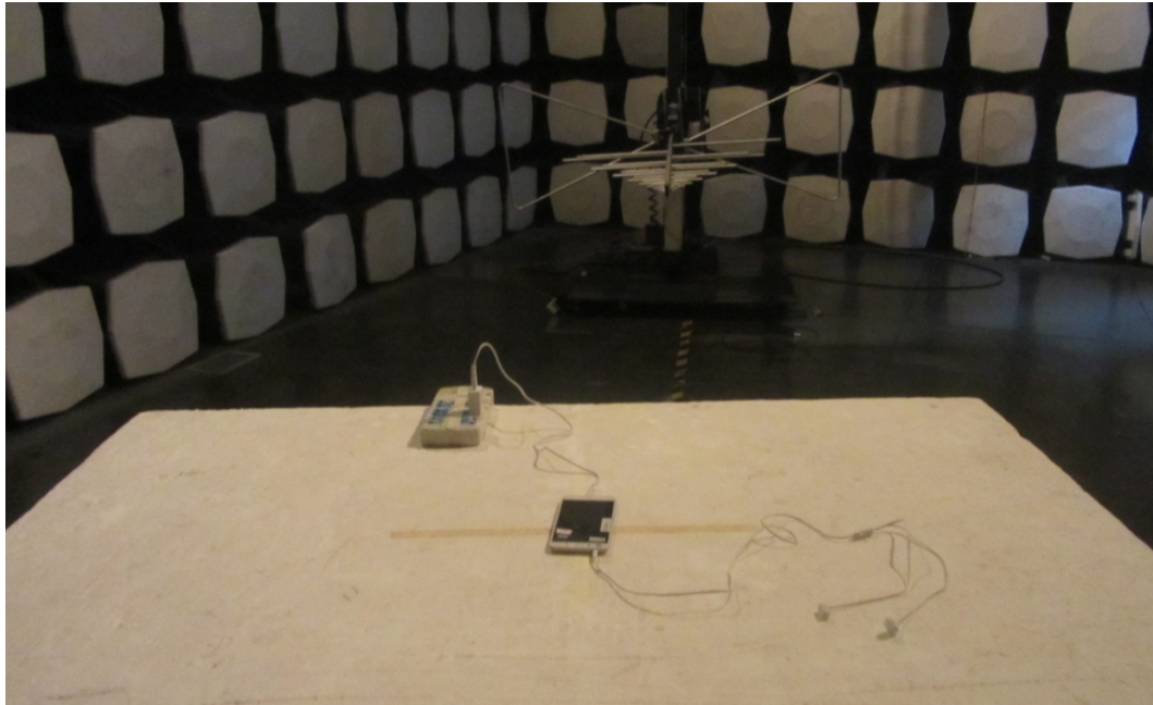
30M Hz-1GHz
