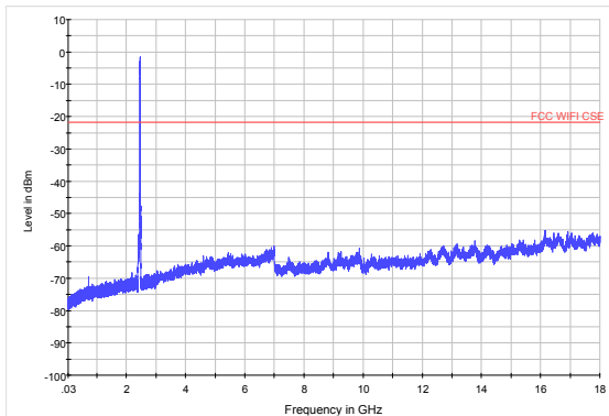
802.11n (HT20) CH11 30MHz to 18GHz
