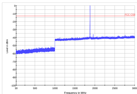
LTE Band 2 1.4MHz CH-Middle 30MHz~3GHz
