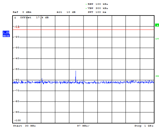
GSM 1900 CH-Low 30MHz~1GHz
