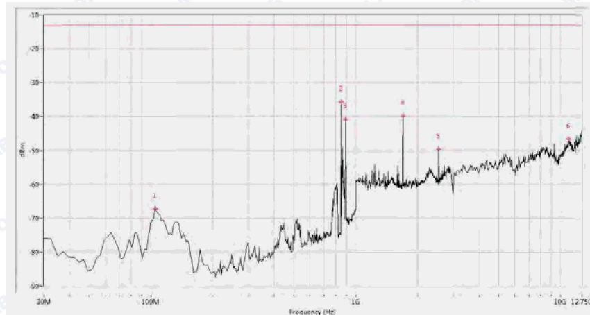
(Plot A.4: GSM 850MHz Channel = 190, Test Antenna Vertical)
