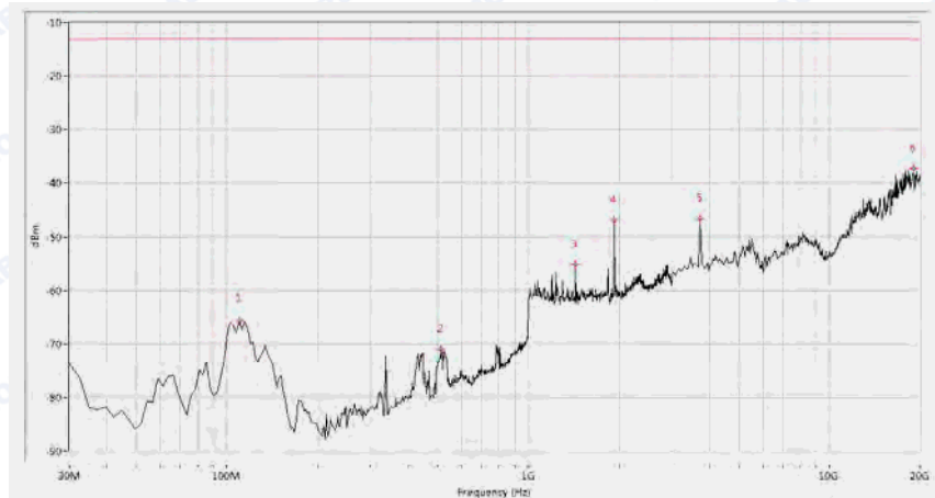
(Plot I.6: HSUPA 850MHz Channel = 4233, Test Antenna Vertical)
