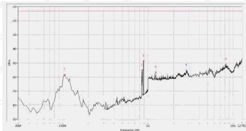
(Plot G.4: HSDPA 850MHz Channel = 4175, Test Antenna Vertical)
