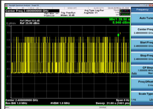
8DPSK,2480,3DH5,Transmission Number
