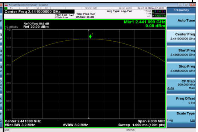
Output Power: 8DPSK,2441MHz,3DH5
