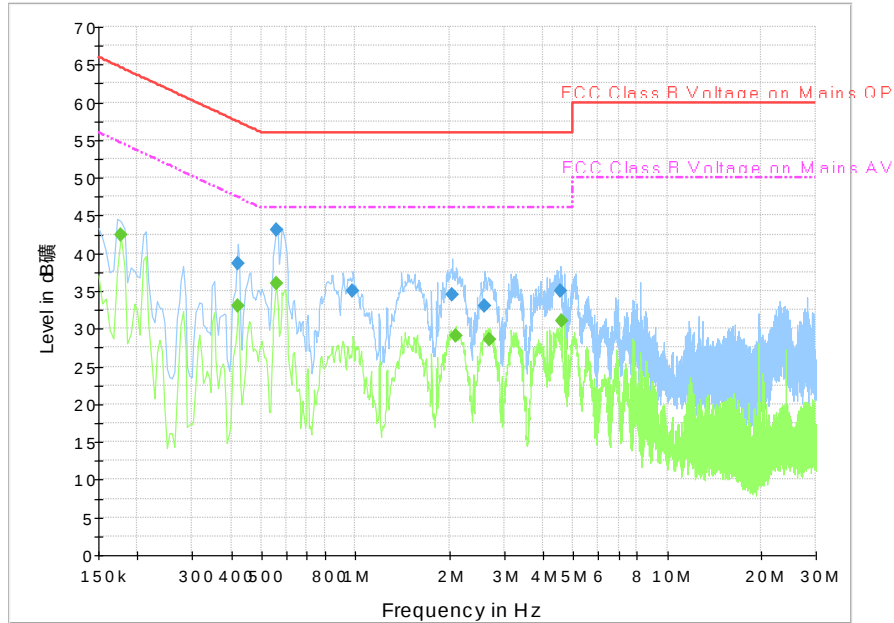
Fig.6 Conducted Emission
