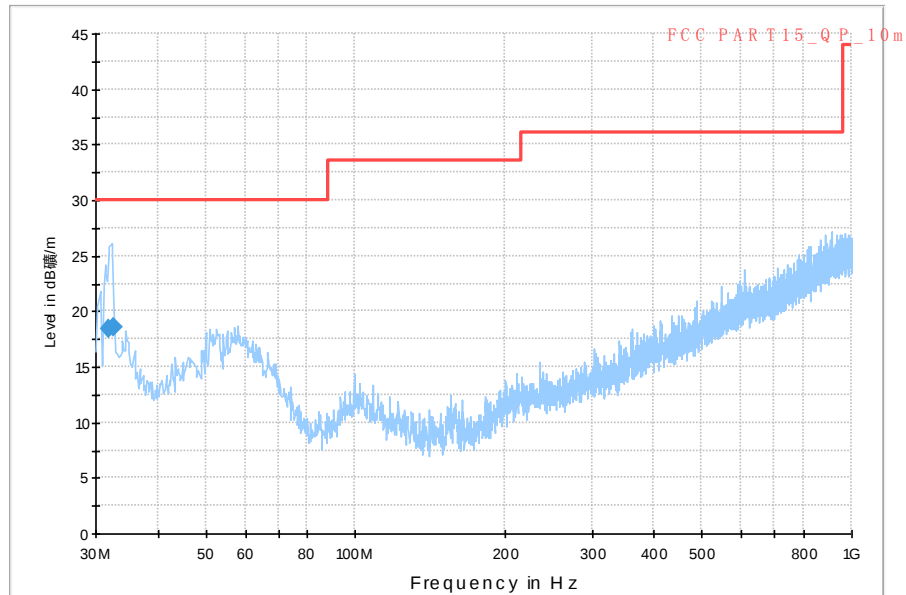
Fig.1 Radiated Emission from 30MHz to 1GHz
