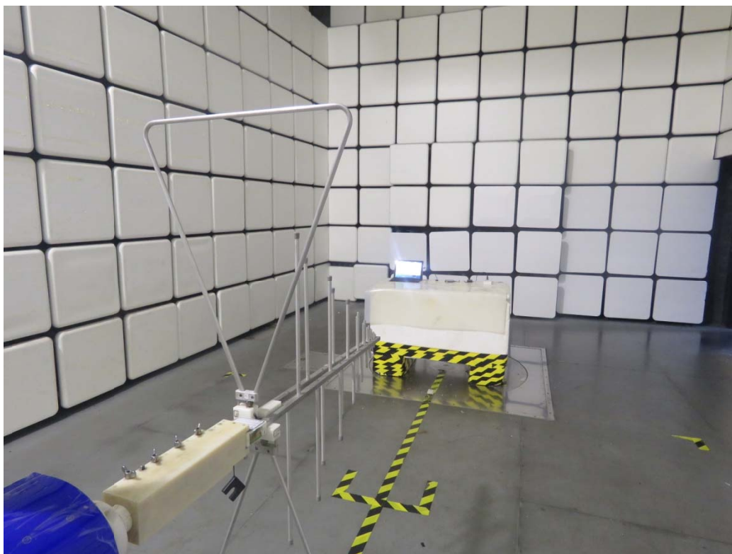
30MHz-1GHz
