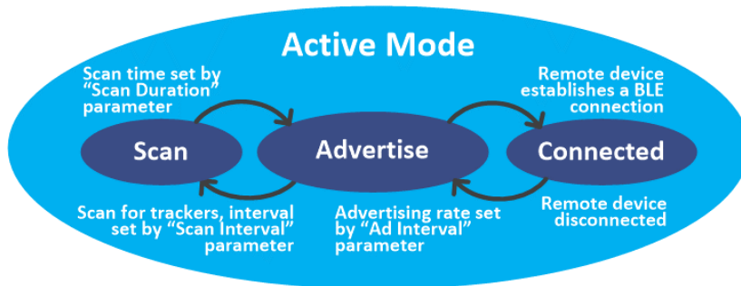
Figure 3 – BLE operations in Active mode
