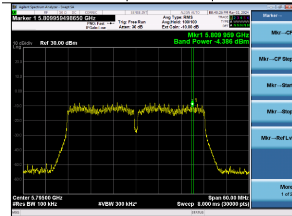
802.11n40 | Channel 159 | MCS7
