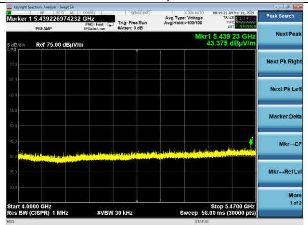
802.11a | Channel 144 | 6 Mbps | Y Plane 4000-5470 MHz | Horizontal
