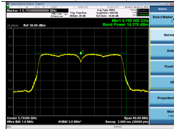
802.11n40 | Channel 151 | MCS7
