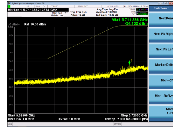
802.11ax40 | Channel 151 | MCS9
