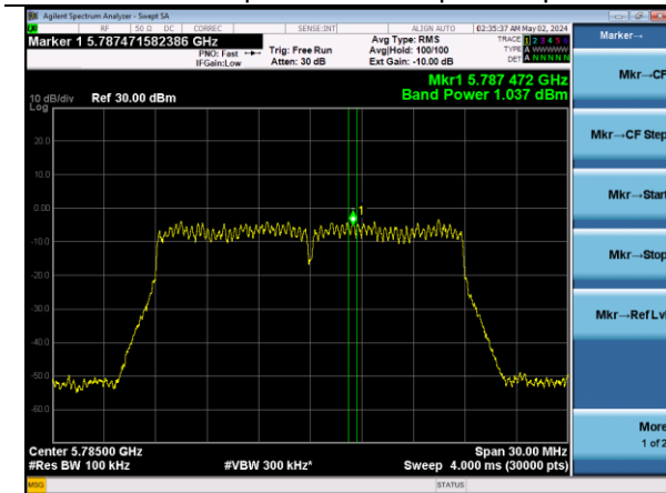
802.11ac20 | Channel 157 | MCS8
