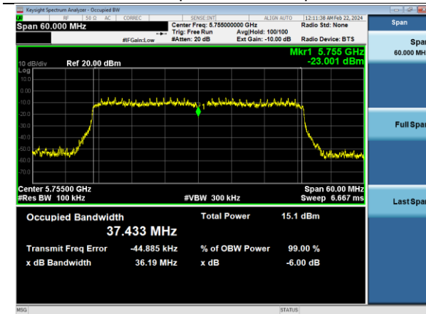
802.11ax40 | Channel 151 | MCS11
