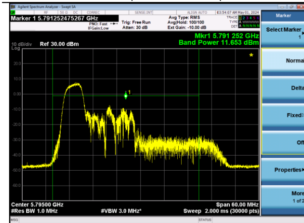
802.11ax40 | Channel 159 | MCS0 | RU 52
