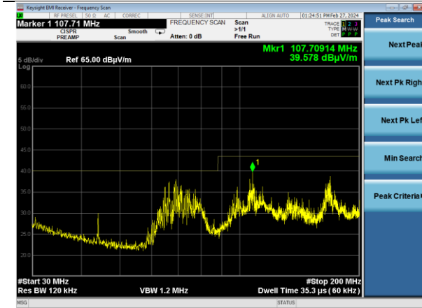
802.11a | Channel 165 | 6 Mbps | Y Plane 30-200 MHz | Horizontal
