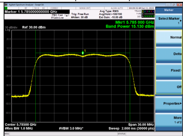
802.11ax20 | Channel 157 | MCS0
