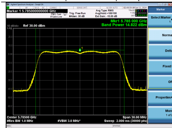
802.11ac20 | Channel 157 | MCS0
