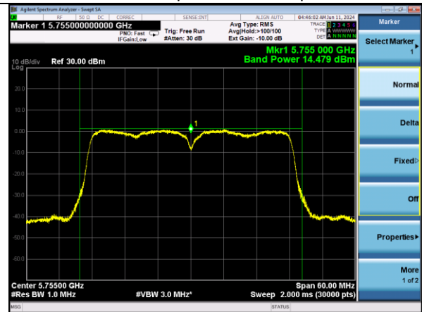
802.11ac40 | Channel 151 | MCS7
