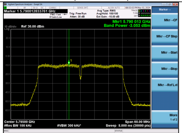
802.11ac40 | Channel 159 | MCS0
