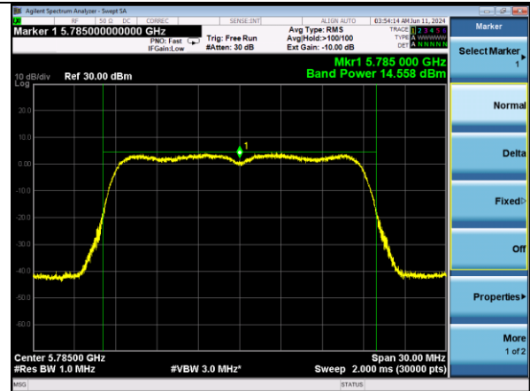
802.11n20 | Channel 157 | MCS7
