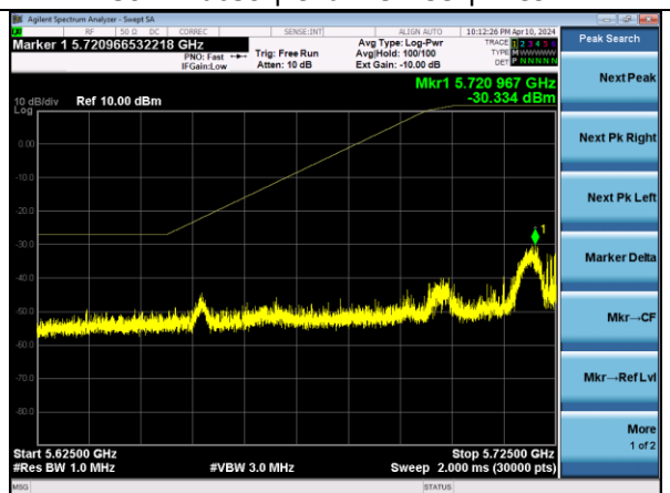
802.11ax20 | Channel 149 | MCS0 | RU26
