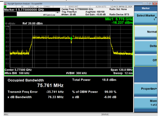
802.11ac80 | Channel 155 | MCS0
