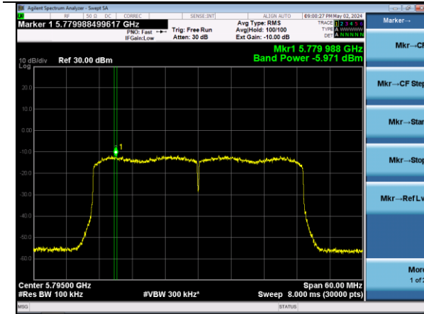
802.11ax40 | Channel 159 | MCS0
