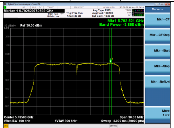
802.11ax20 | Channel 157 | MCS0
