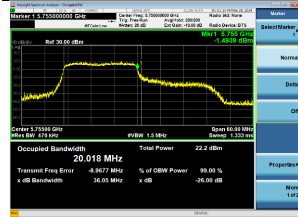
802.11ax40 | Channel 151 | MCS0 | RU Tone 242 Index 61
