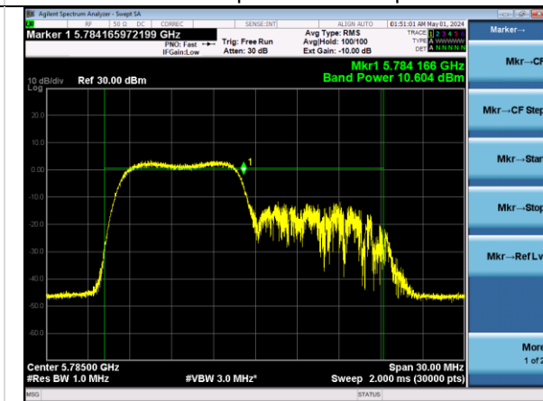
802.11ax20 | Channel 157 | MCS0 | RU106
