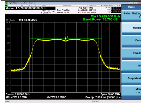
802.11a | Channel 157 | 6 Mbps
