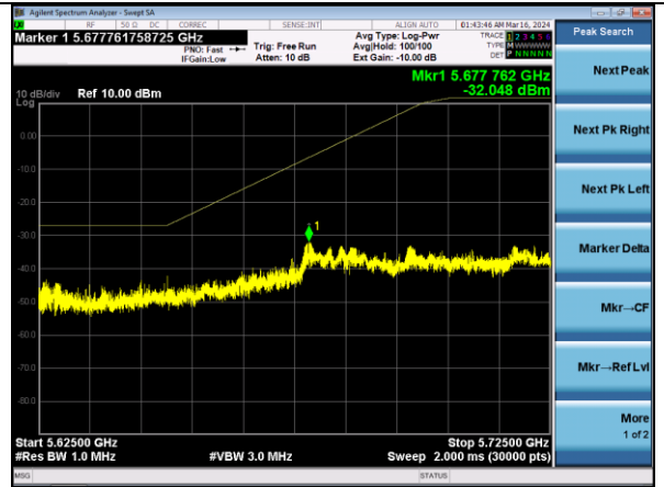
802.11ac80 | Channel 155 | MCS7
