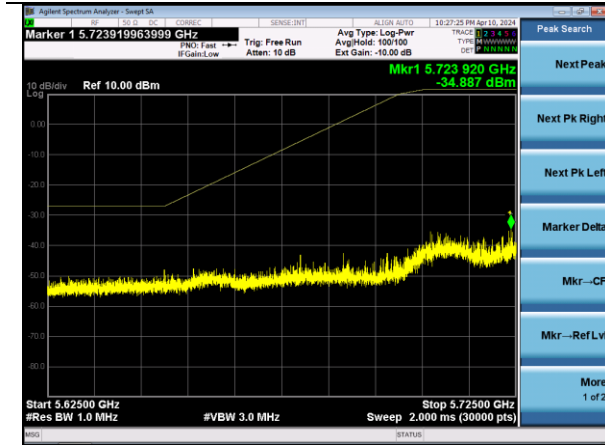
802.11ax40 | Channel 151 | MCS0 | RU106
