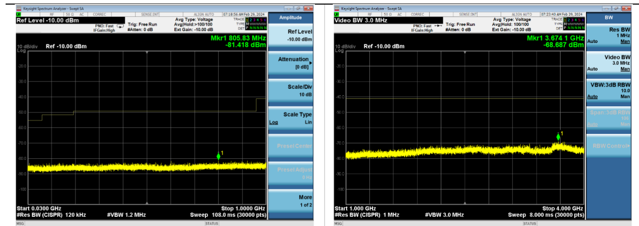
802.11a | Channel 149 | 6 Mbps | 1000-4000 MHz
