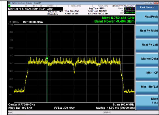
802.11ac80 | Channel 155 | MCS8
