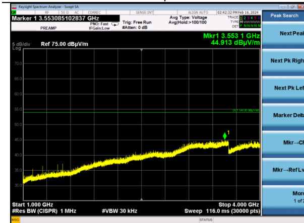
802.11a | Channel 157 | 6 Mbps 1000-4000 MHz | Horizontal
