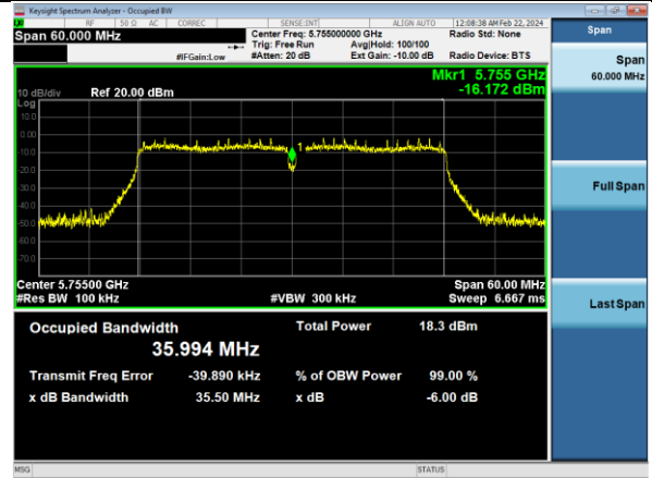
802.11ac40 | Channel 151 | MCS0
