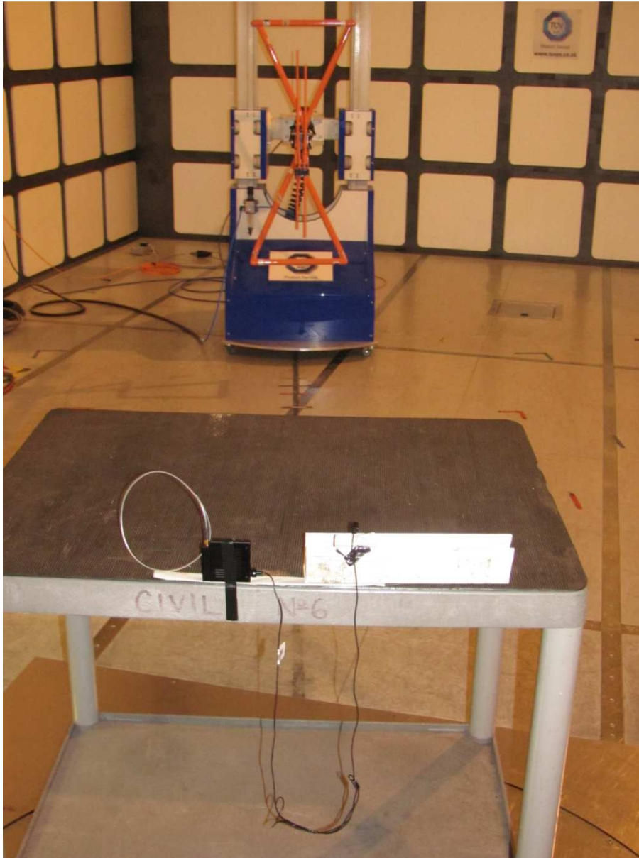
Radiated Emissions and ERP
