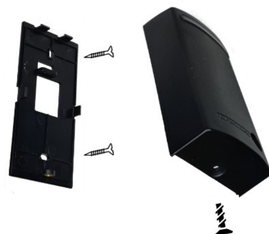
Mounting
