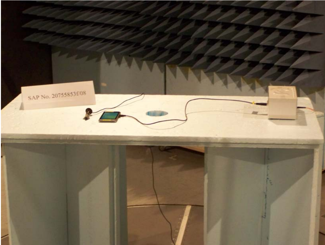
Photograph 3: Radiated field strength: USB-cable
