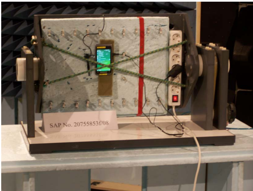
Photograph 2: Radiated field strength – AC/DC Adapter
