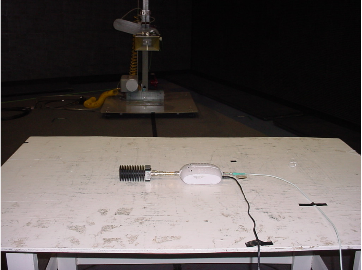
Figure 3: Spurious Emissions
