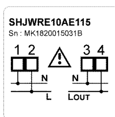
115V, connections
