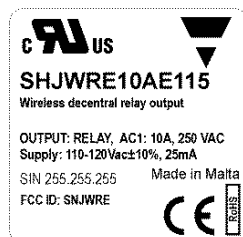
115V, product
