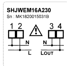
230V, connections
