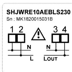
230V, black, light switch, connections
