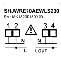
230V, white, light switch, connections
