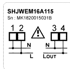
115V, connections
