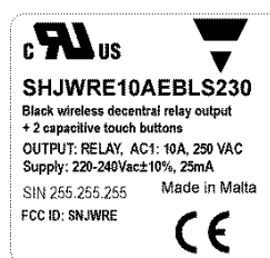
230V, black, light switch, product
