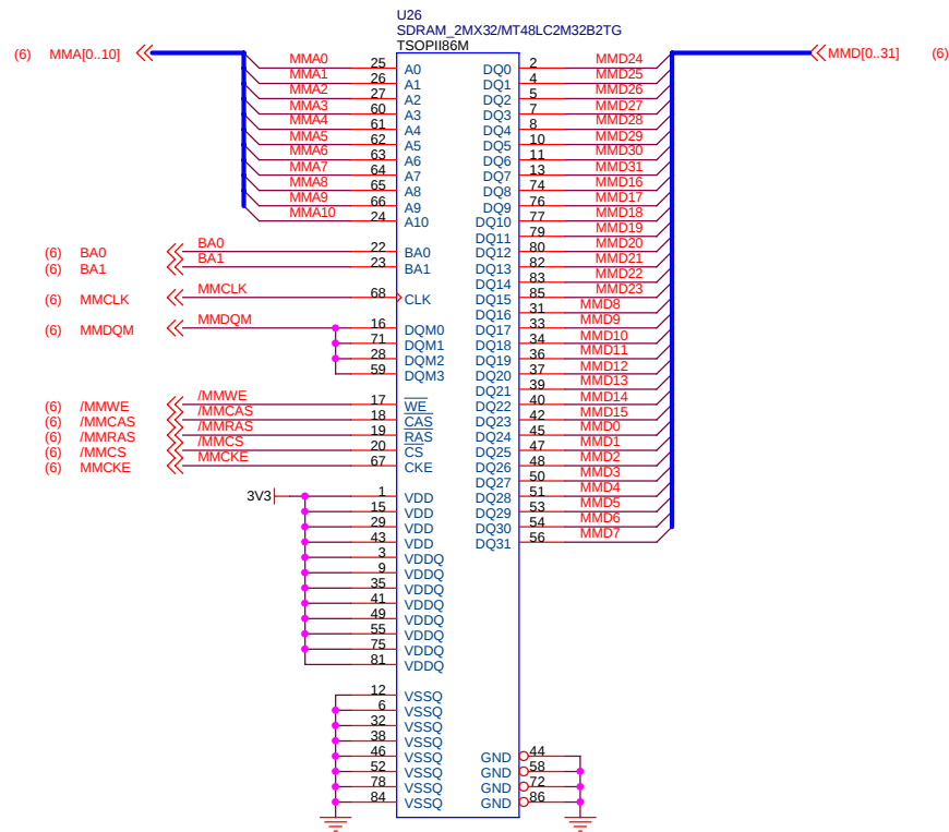
SDRAM(64Mbit)
