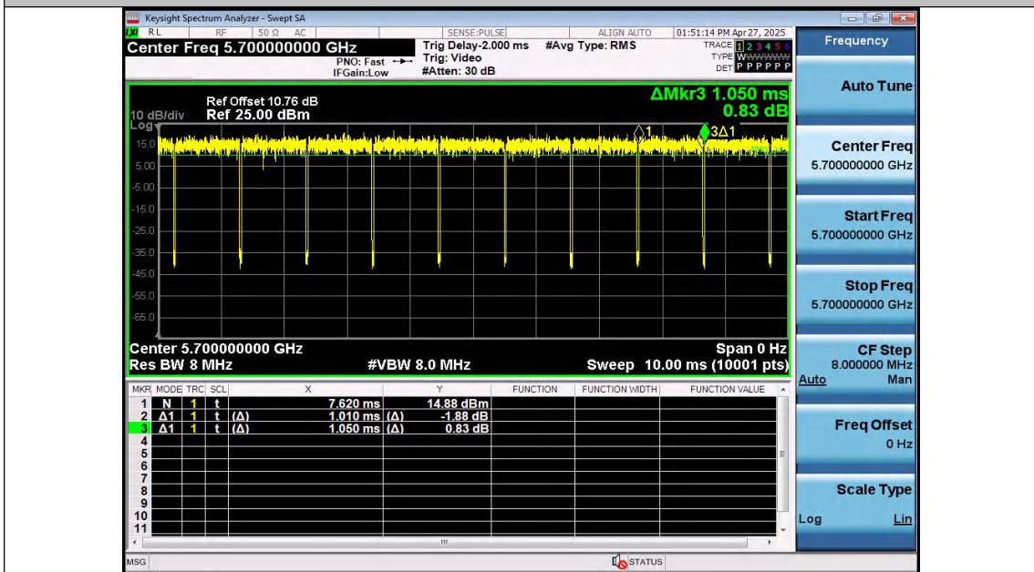
NTNV-11AX20SISO-Ant1-5700
