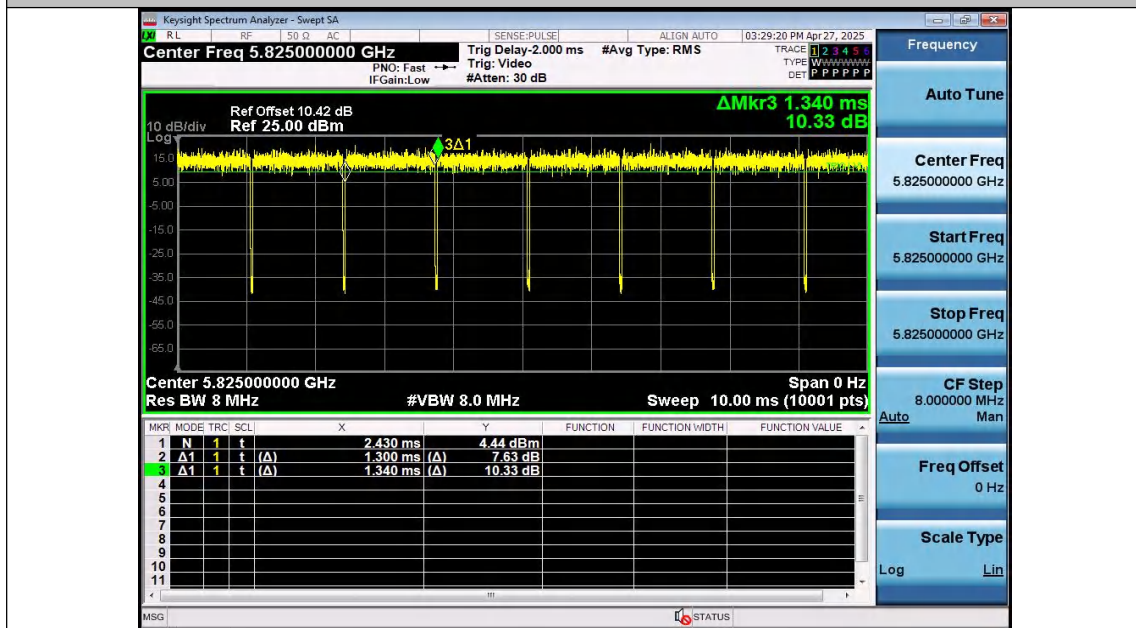
NTNV-11N20SISO-Ant2-5825
