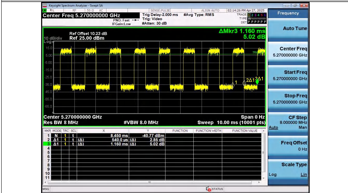
NTNV-11AX40SISO-Ant1-5270
