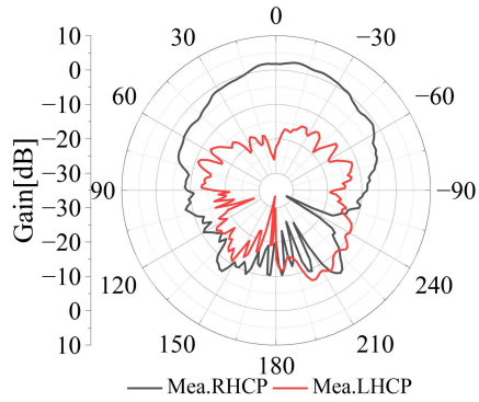
Ant2_8GHz_xoz Gain: 2.55 dBi
