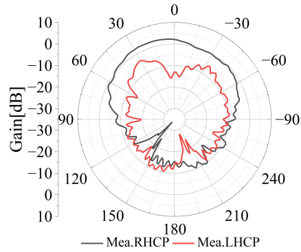
Ant2_8GHz_yoz Gain: 2.56 dBi
