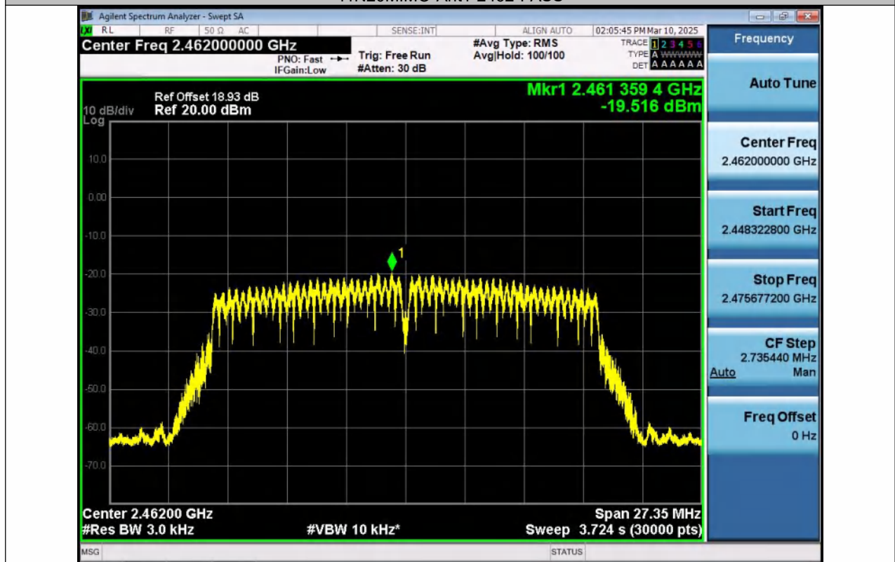
11N20MIMO-Ant2-2462-PASS
