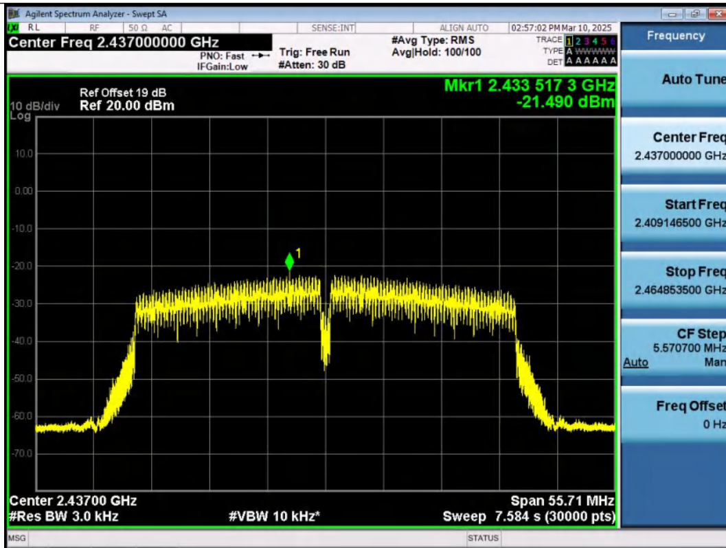
11N40MIMO-Ant1-2437-PASS
