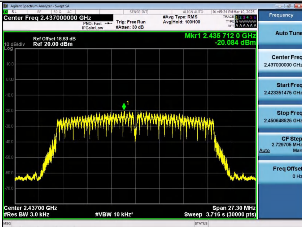
11N20MIMO-Ant2-2437-PASS
