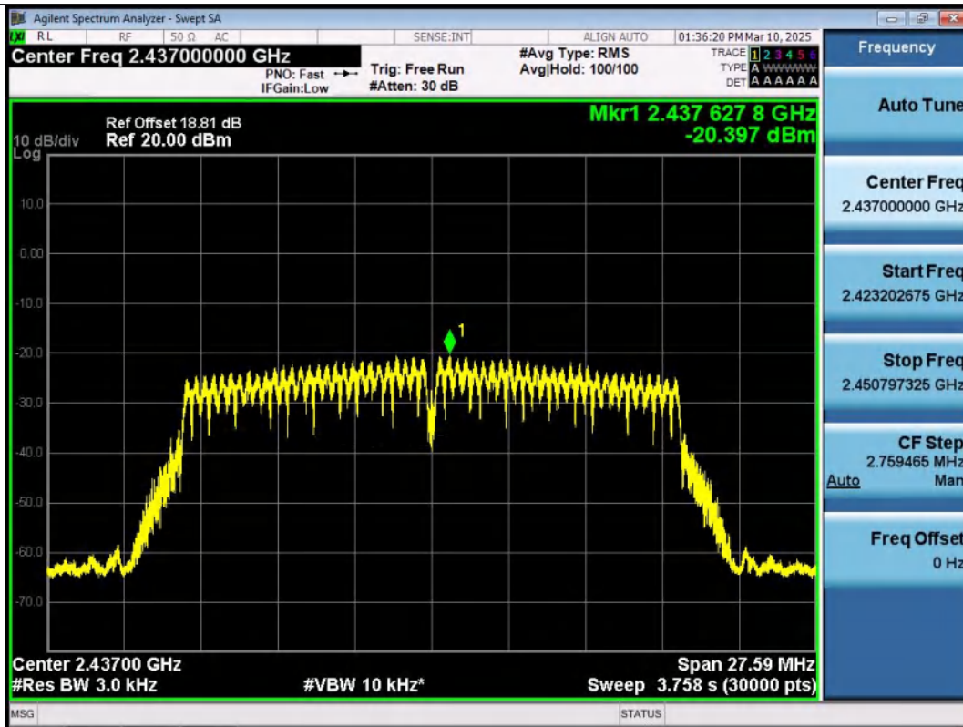
11N20MIMO-Ant1-2437-PASS
