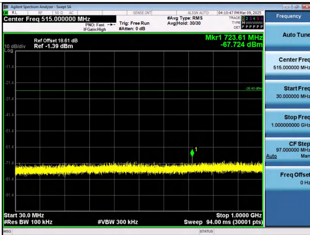
11B-Ant1-2437-30~1000-PASS
