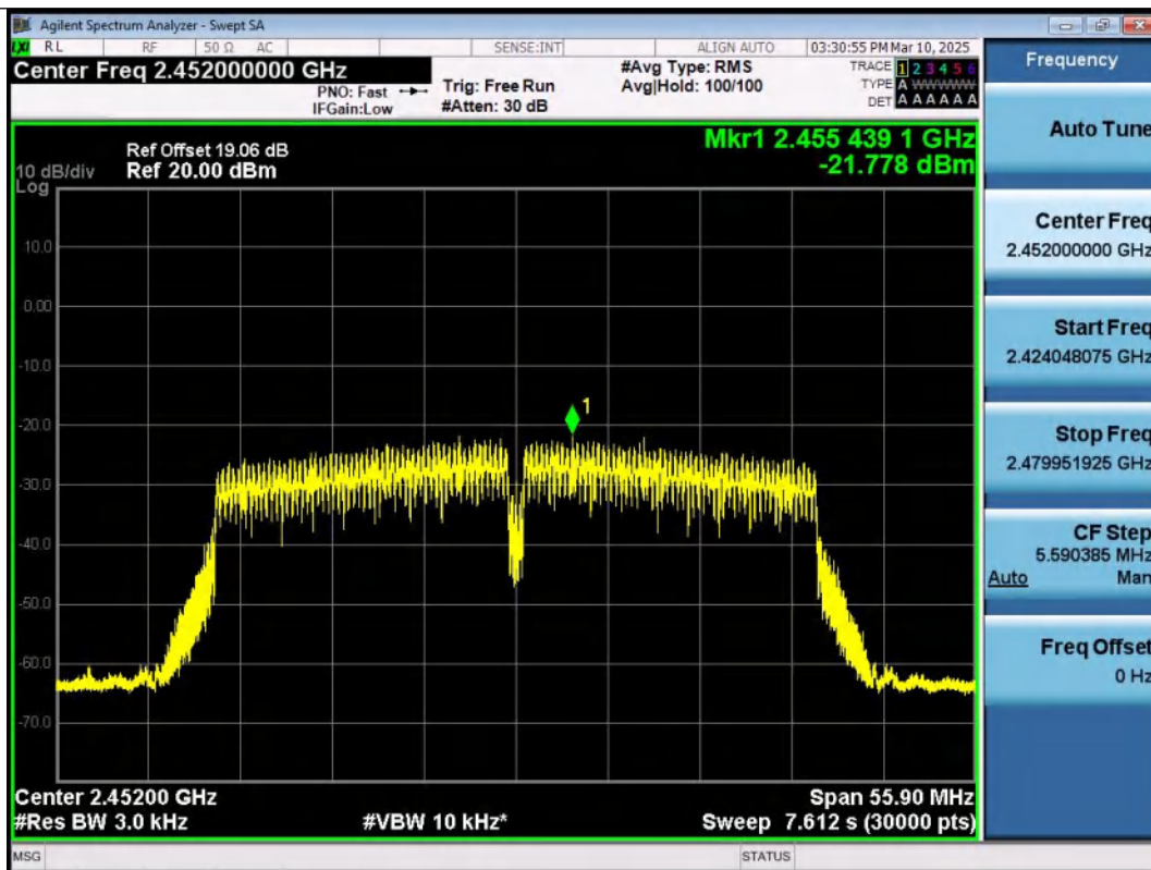
11N40MIMO-Ant1-2452-PASS
