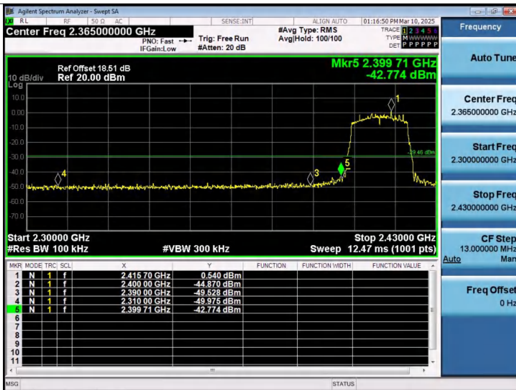
11N20MIMO-Ant1-2412-PASS
