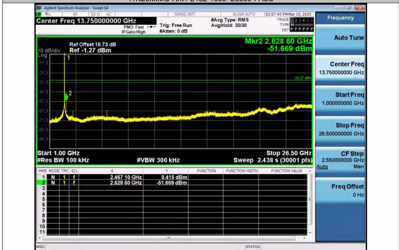
11N20MIMO-Ant2-2462-1000~26500-PASS
