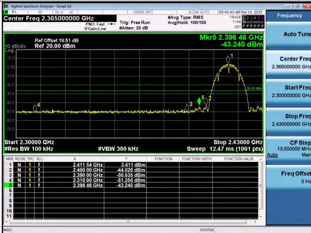
11B-Ant2-2412-PASS
