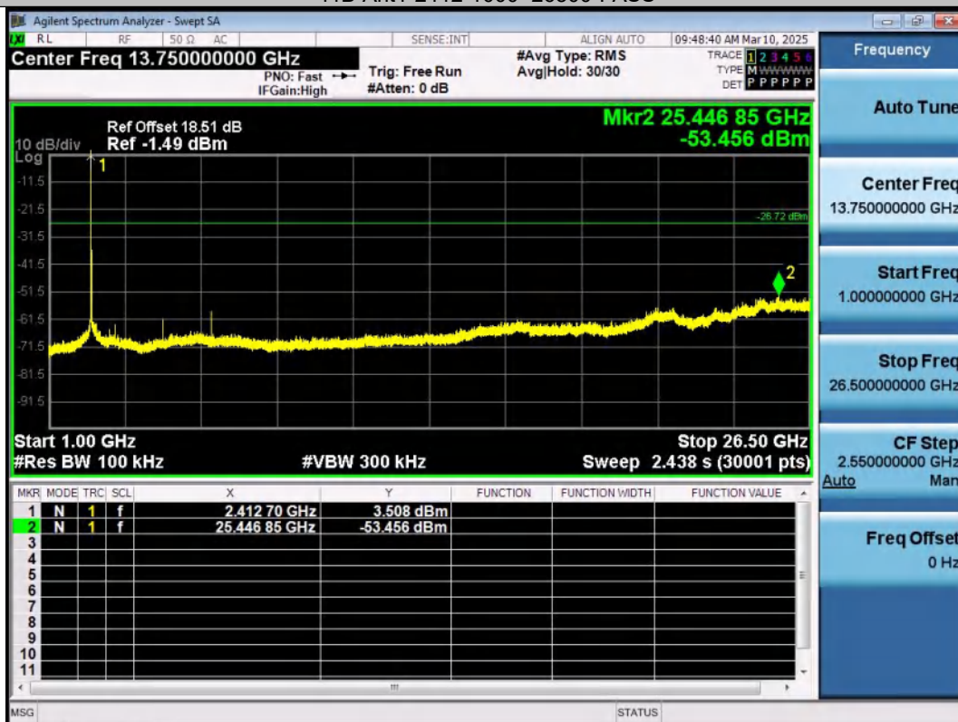
11B-Ant2-2412-1000~26500-PASS
