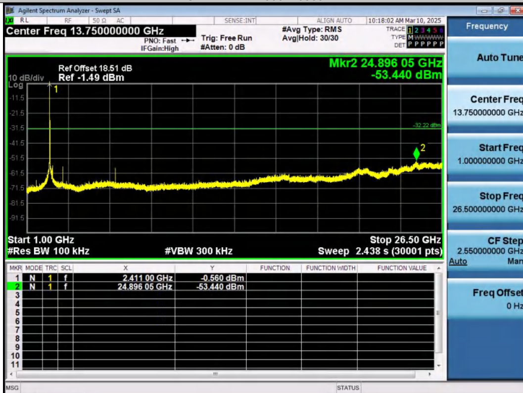
11G-Ant2-2412-1000~26500-PASS
