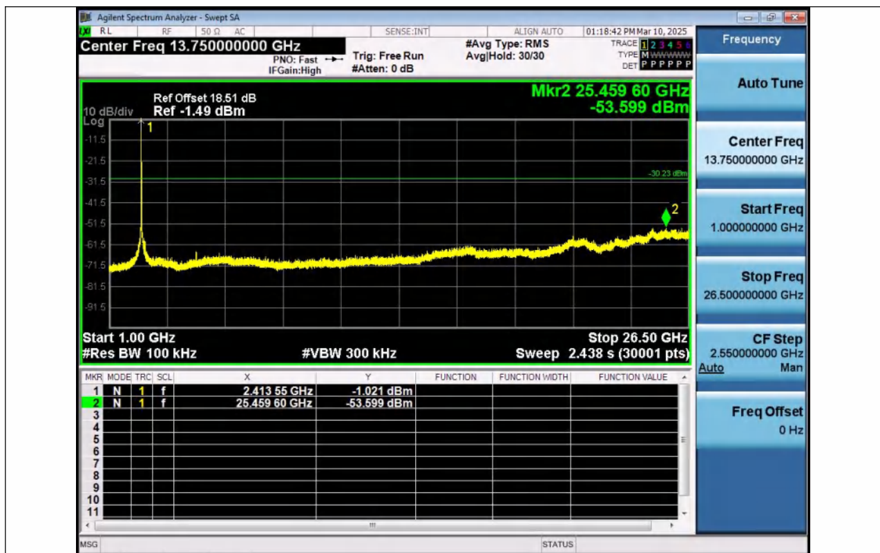
11N20MIMO-Ant1-2412-1000~26500-PASS
