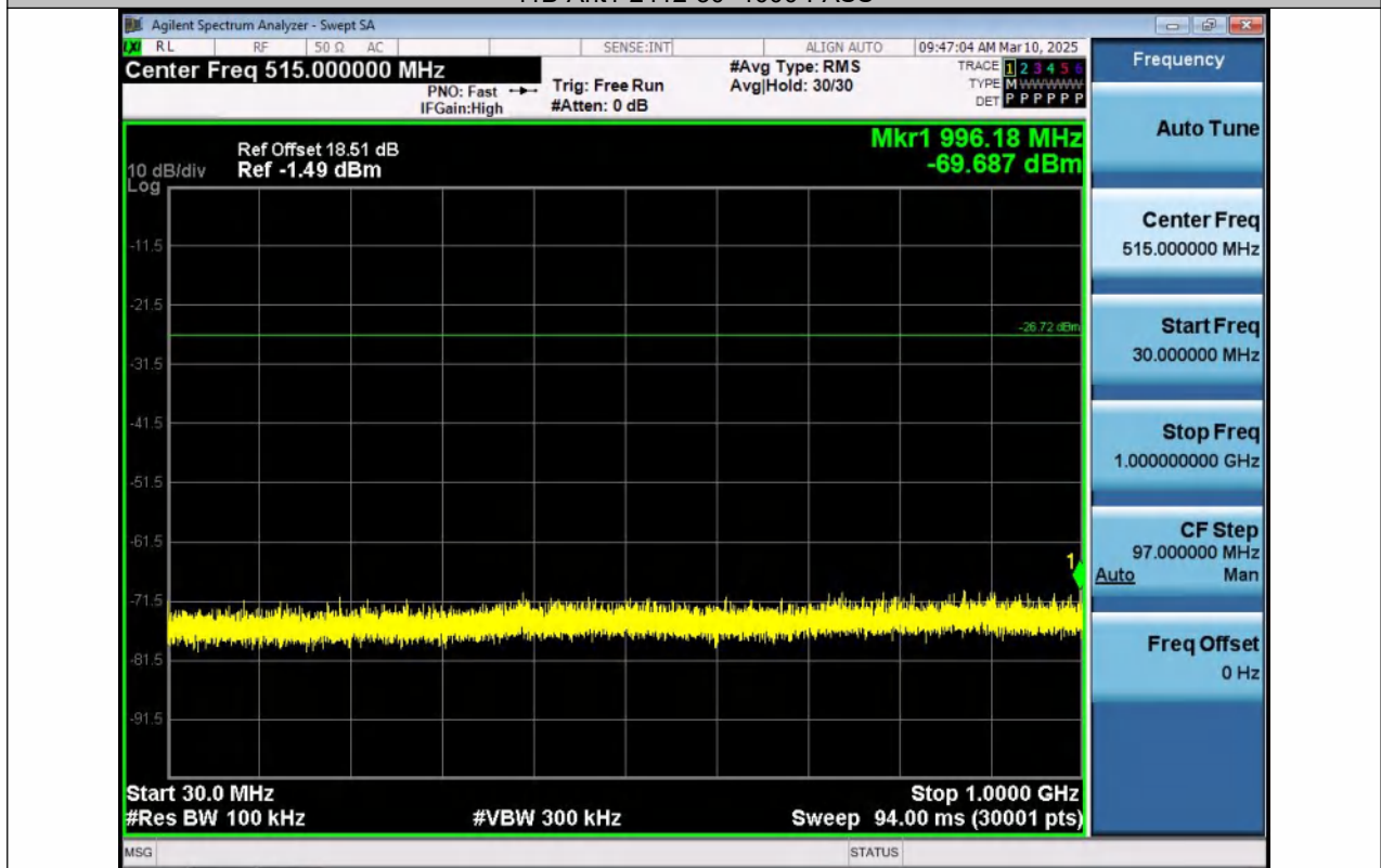
11B-Ant2-2412-30~1000-PASS
