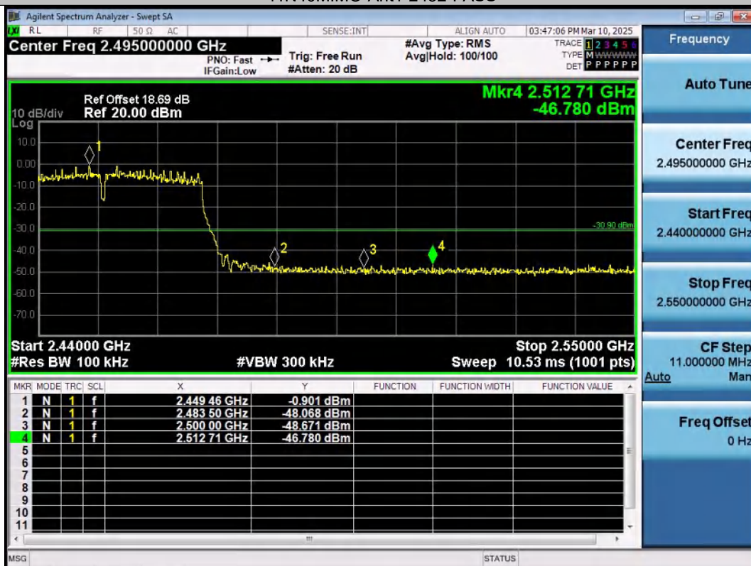
11N40MIMO-Ant2-2452-PASS
