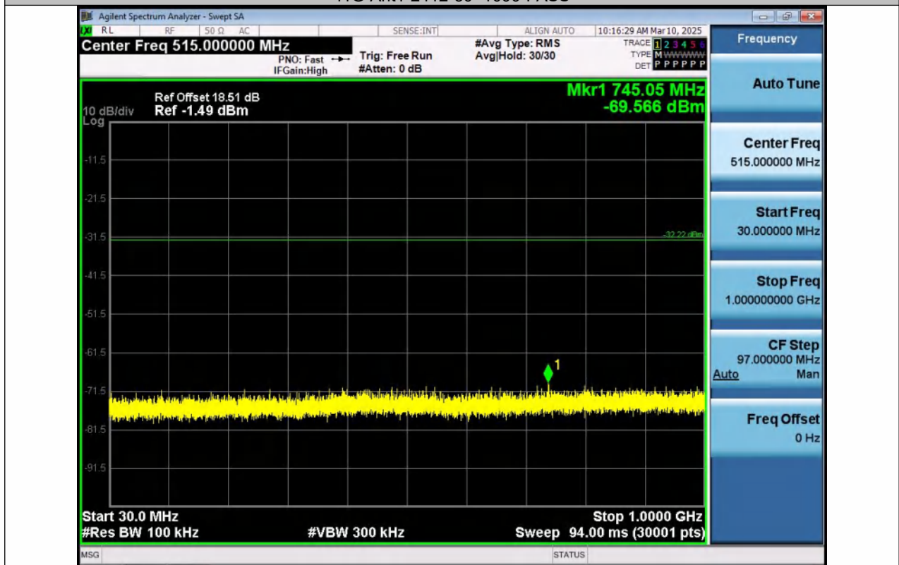
11G-Ant2-2412-30~1000-PASS
