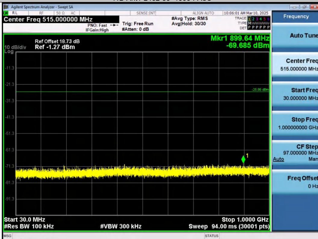
11B-Ant2-2462-30~1000-PASS
