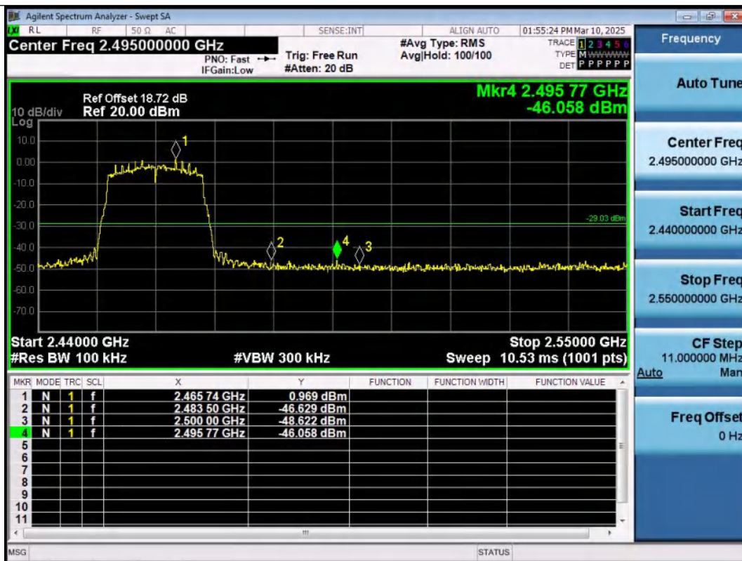
11N20MIMO-Ant1-2462-PASS
