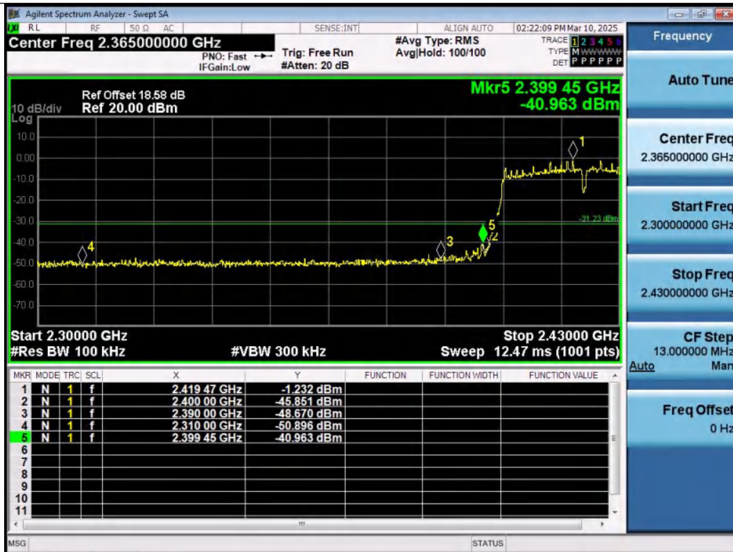
11N40MIMO-Ant1-2422-PASS
