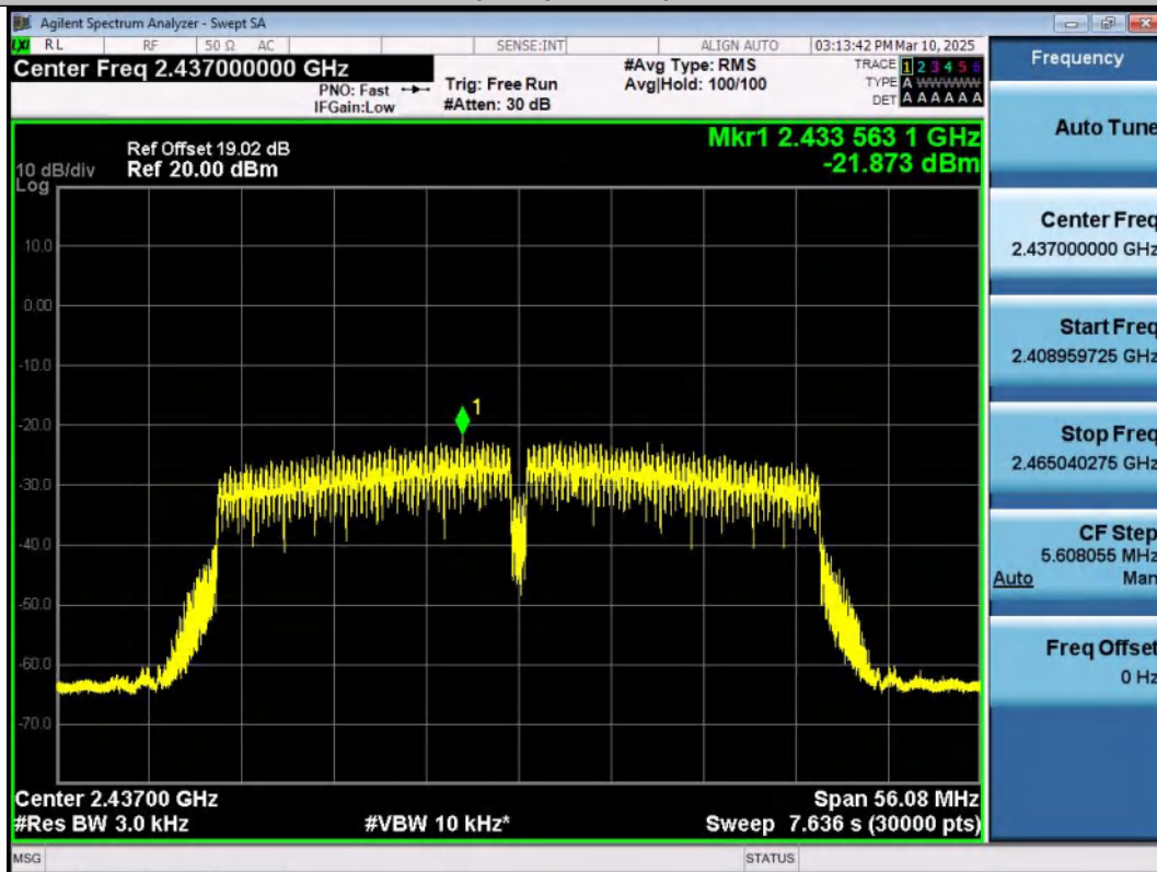
11N40MIMO-Ant2-2437-PASS
