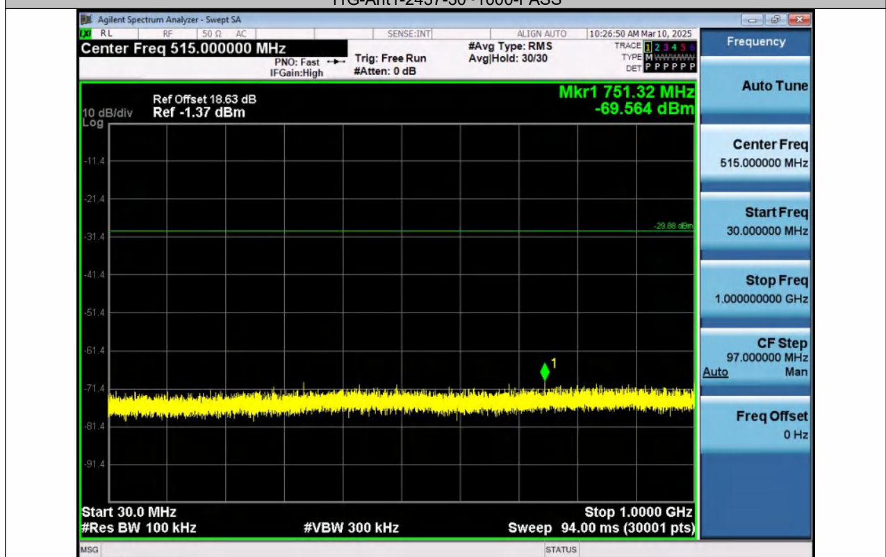
11G-Ant2-2437-30~1000-PASS
