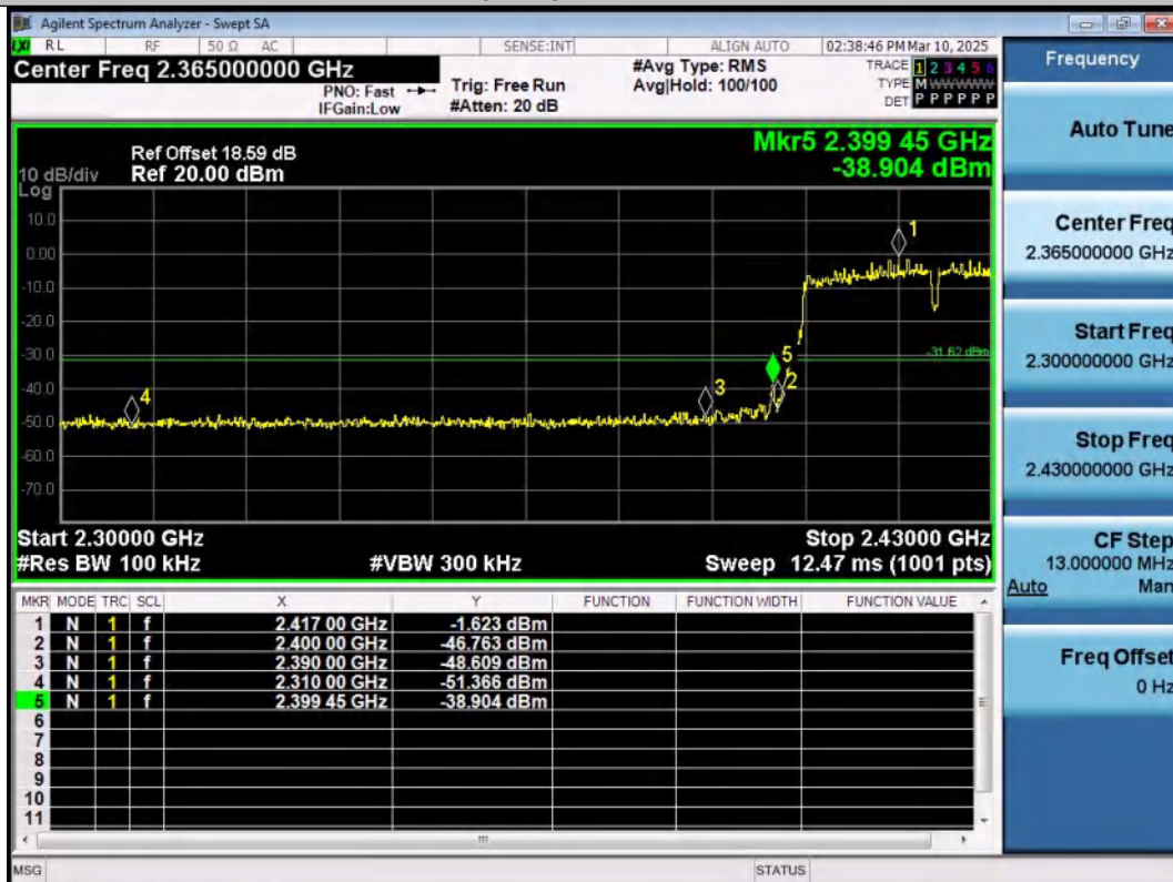
11N40MIMO-Ant2-2422-PASS
