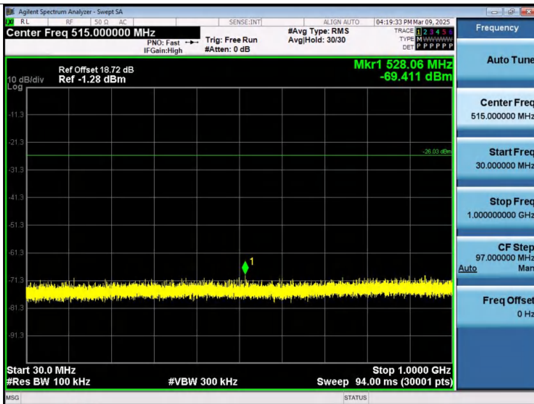
11B-Ant1-2462-30~1000-PASS
