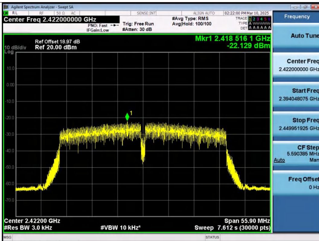
11N40MIMO-Ant1-2422-PASS
