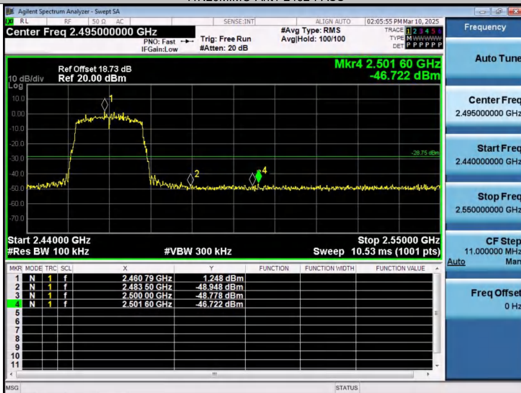
11N20MIMO-Ant2-2462-PASS
