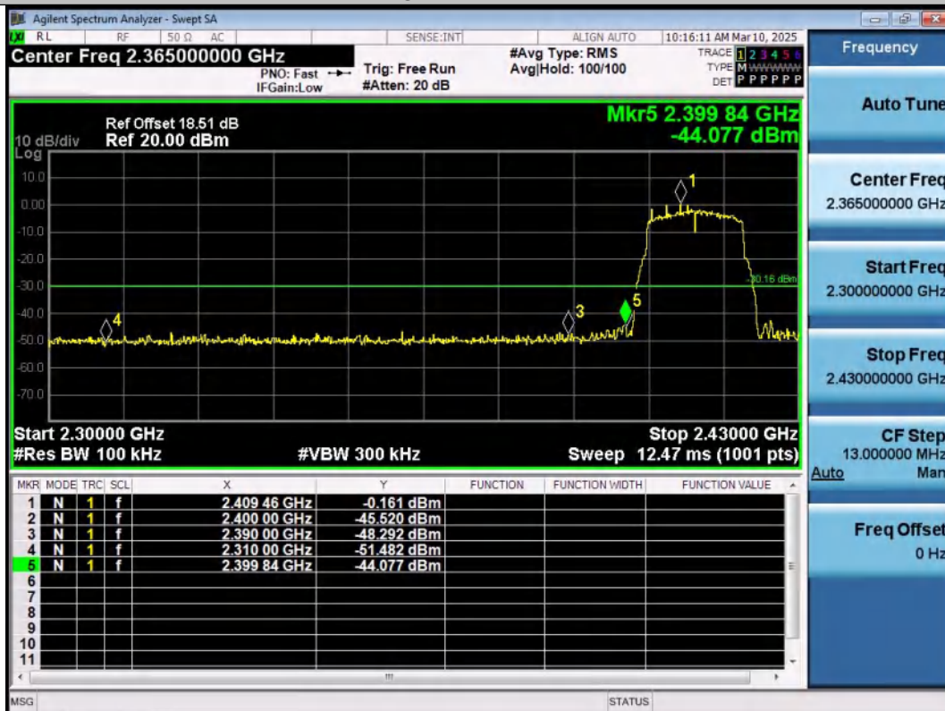
11G-Ant2-2412-PASS
