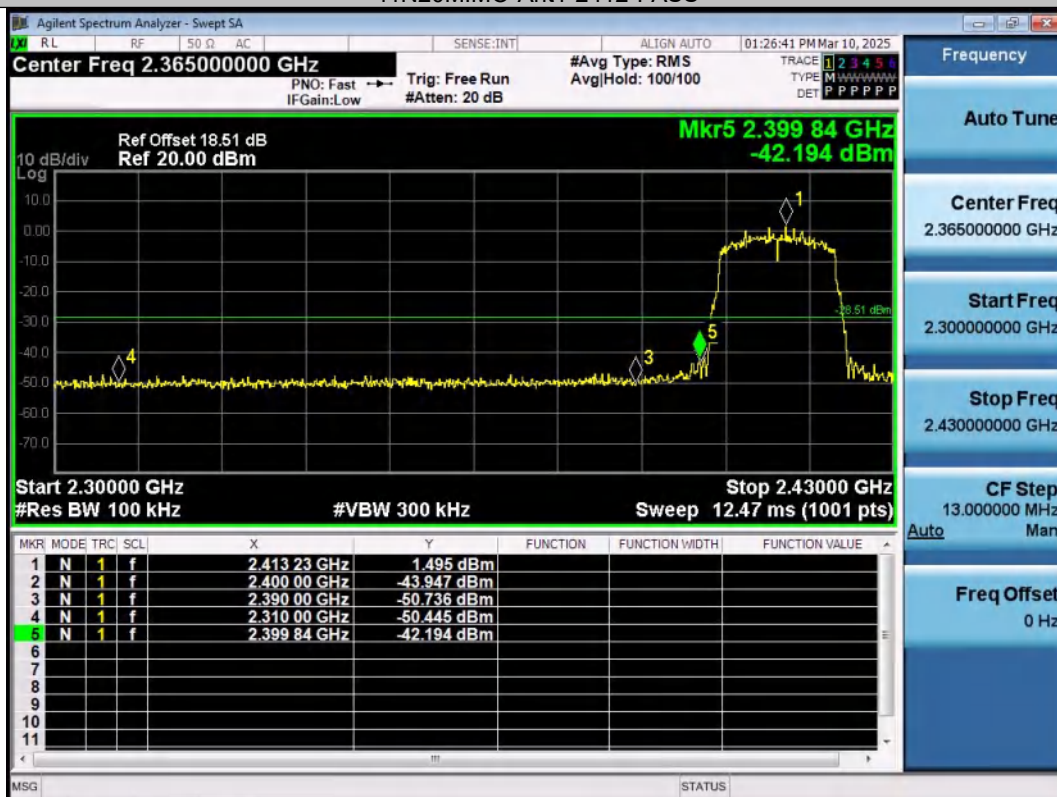
11N20MIMO-Ant2-2412-PASS
