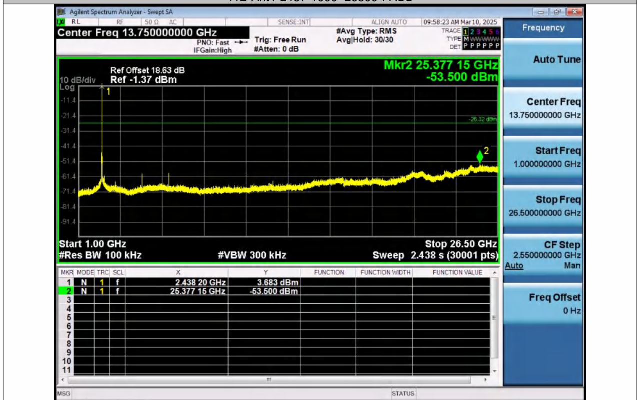
11B-Ant2-2437-1000~26500-PASS
