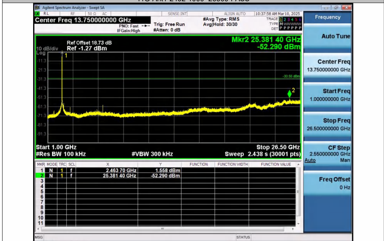
11G-Ant2-2462-1000~26500-PASS
