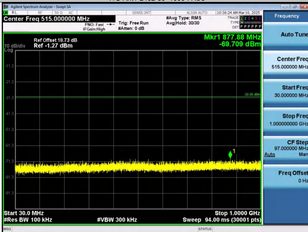
11G-Ant2-2462-30~1000-PASS
