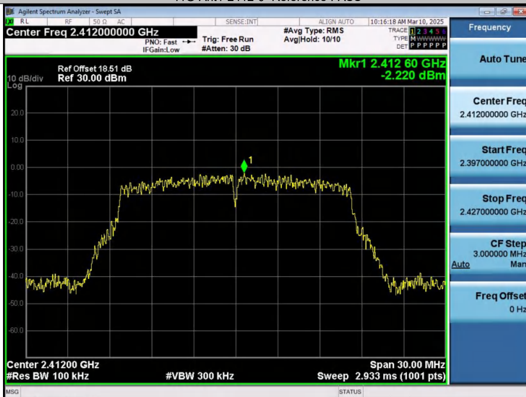
11G-Ant2-2412-0~Reference-PASS
