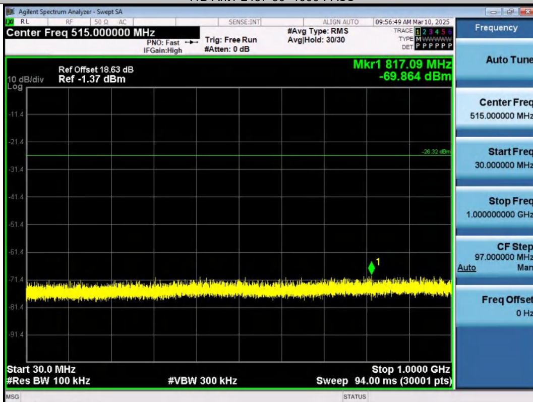
11B-Ant2-2437-30~1000-PASS
