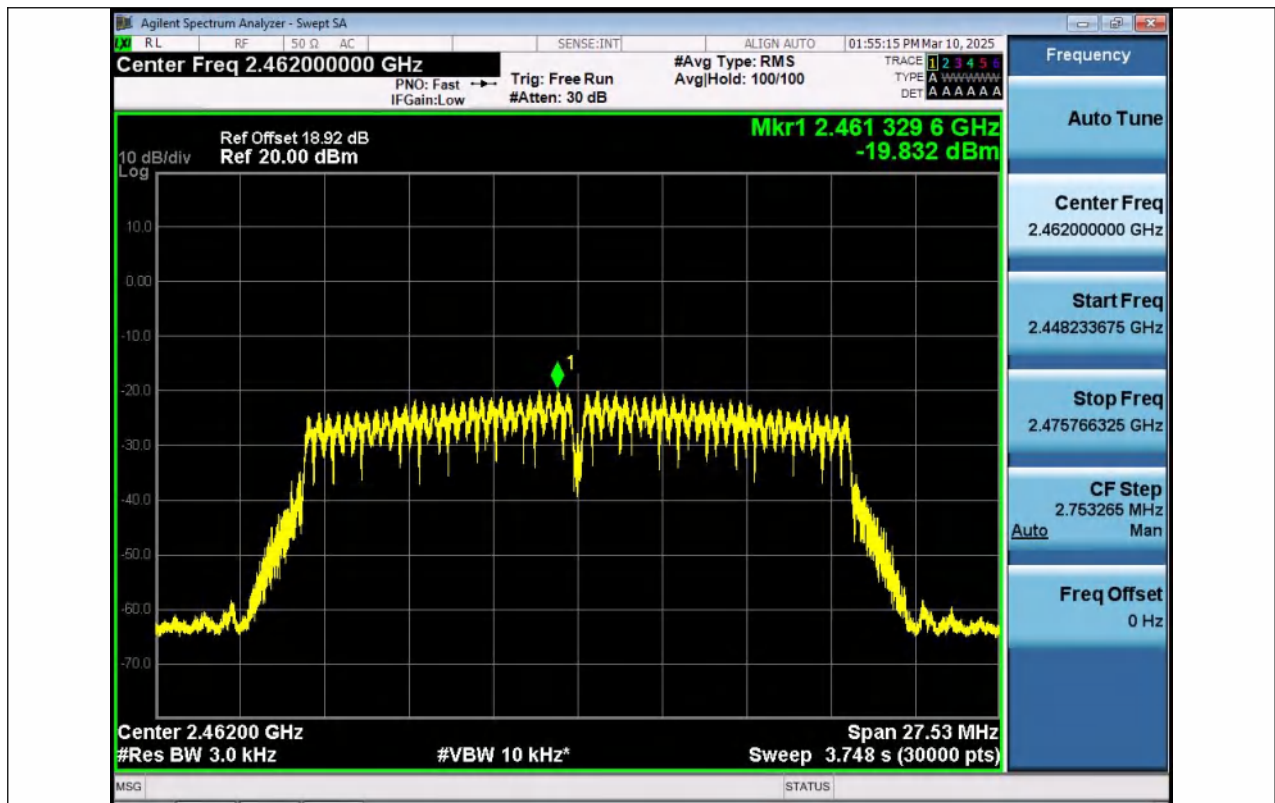
11N20MIMO-Ant1-2462-PASS
