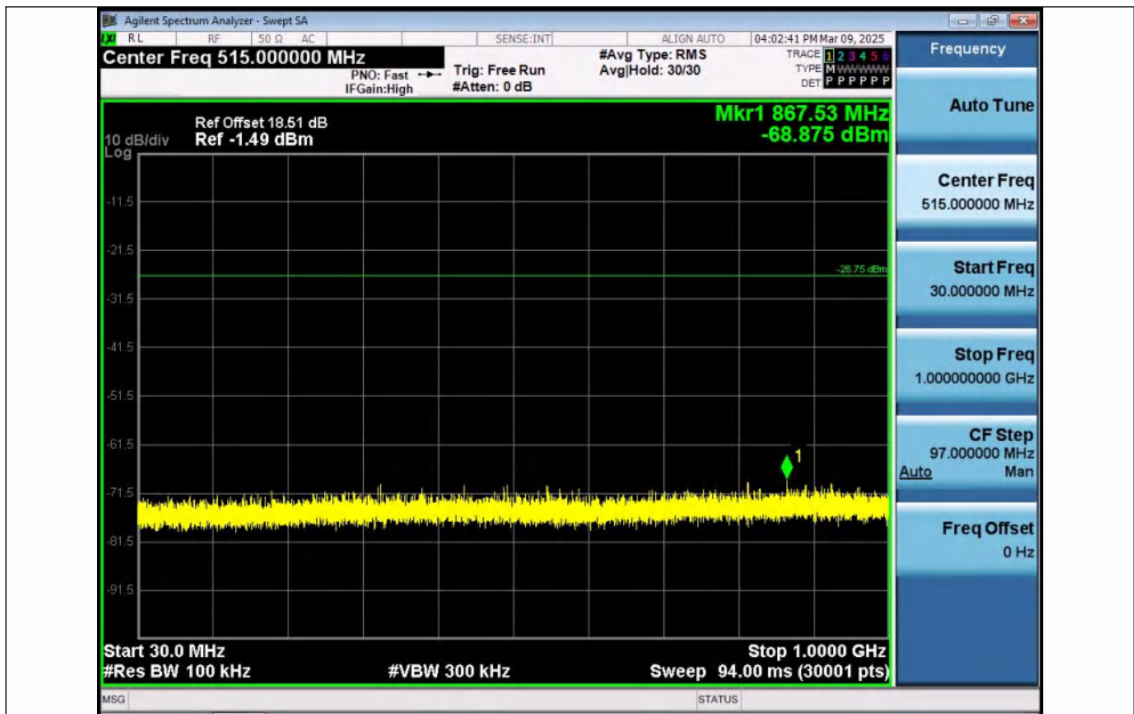
11B-Ant1-2412-30~1000-PASS
