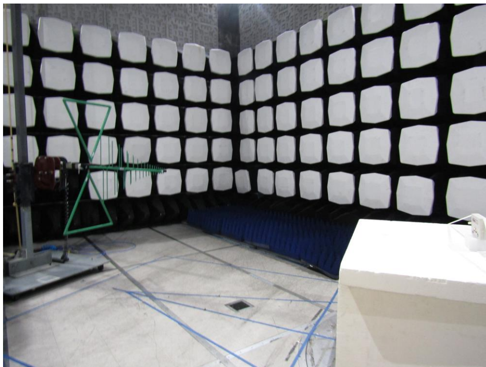
Figure A-2: Test Setup – Radiated Emissions <1GHz
