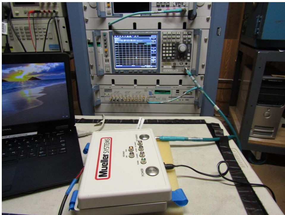
Figure A-4: Test Setup – Antenna Port Measurement
