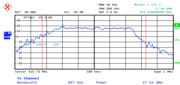
Figure 7.3.2-2: RF Output Power - Middle Channel
