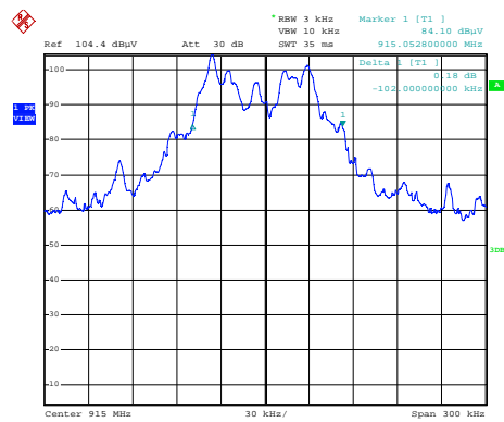
Figure 7.3.2-2: 20dB Bandwidth Plot – 915MHz
