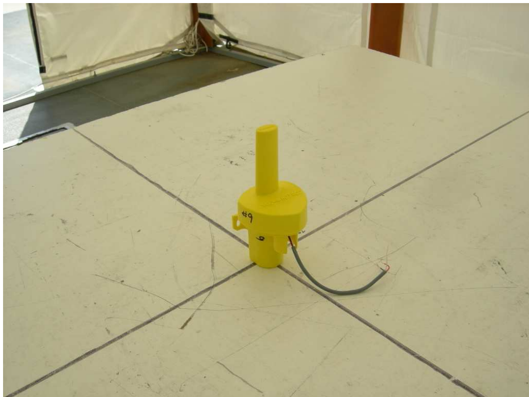
Figure 2: Radiated Emissions – Table Top
