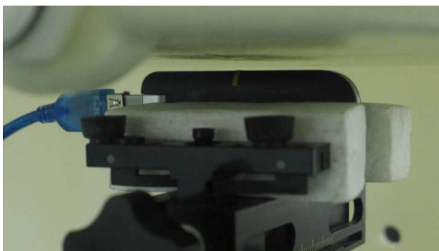
USB cable plug-in for Configuration 4 (Vertical Back with Phantom 5mm Gap)
