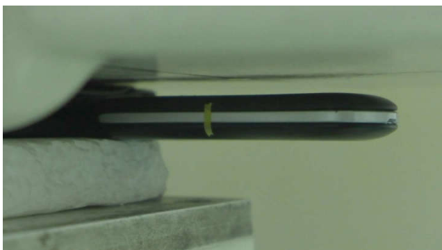
Direct Laptop Plug-in for Configuration 1 (Horizontal Up with Phantom 5mm Gap)
