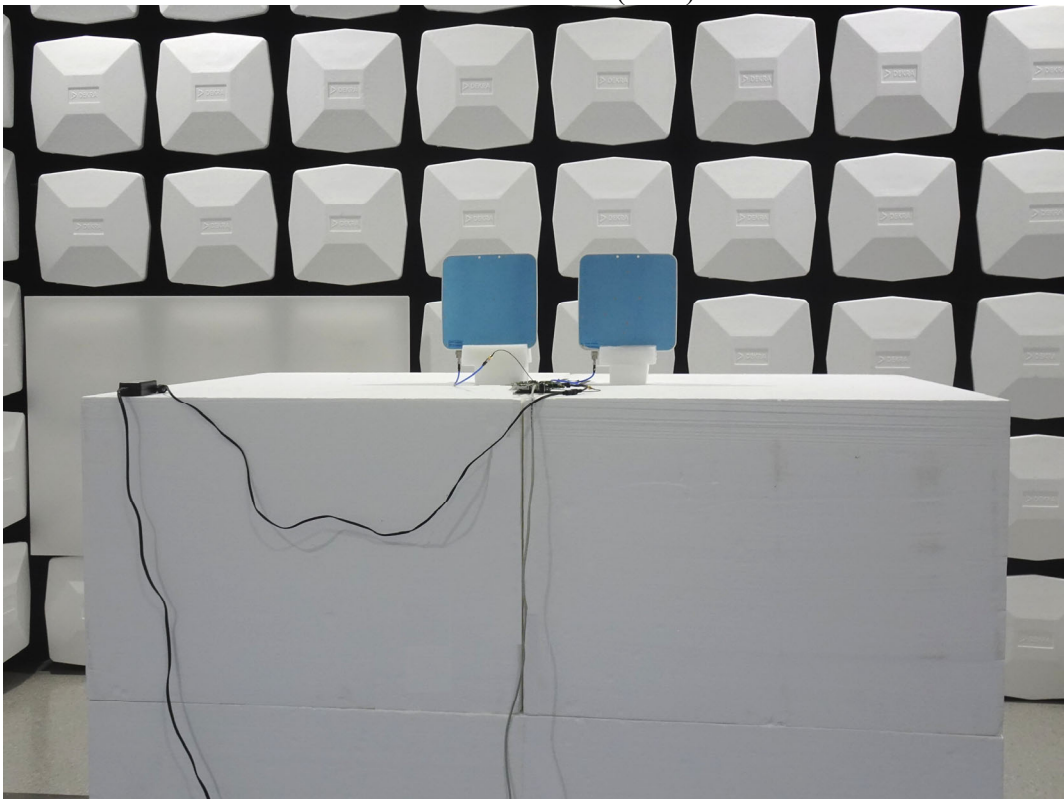
Back View of Radiated Test (Horn) - Panel
