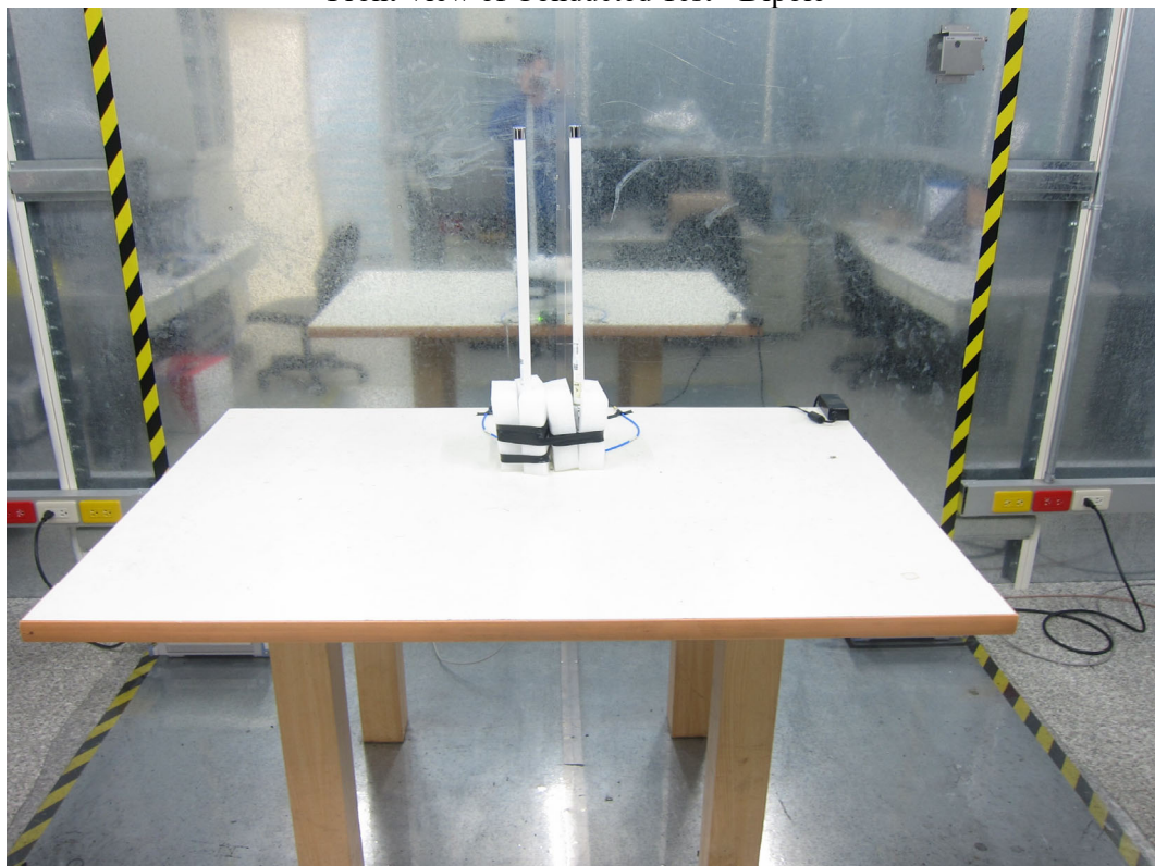
Front View of Conducted Test - Dipole
