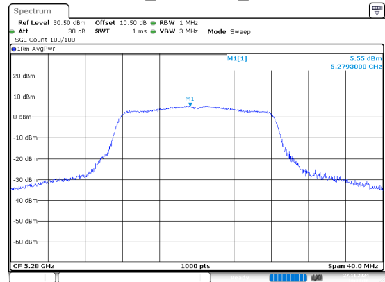
802.11a_5280MHz_Chain 0
