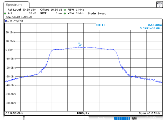
802.11a_5580MHz_Chain 0
