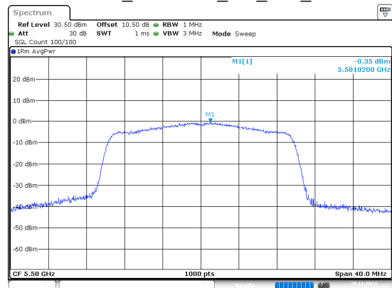
802.11ax20_5580MHz_RU_Full_Chain 1
