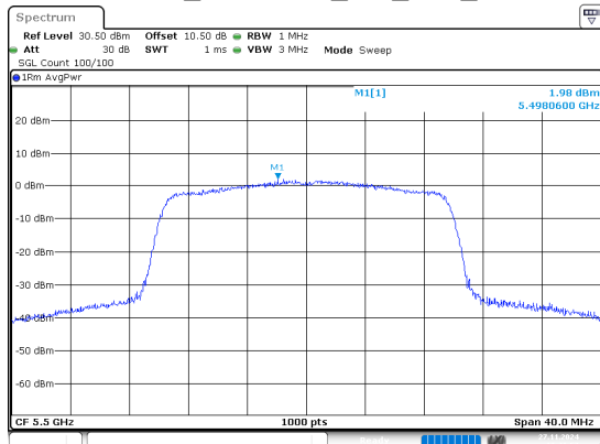
802.11ax20_5500MHz_RU_Full_Chain 0
