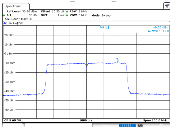
802.11ac80_5690MHz_Chain 0
