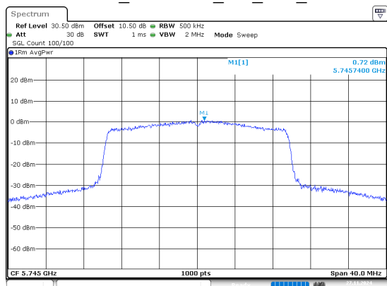
802.11ax20_5745MHz_RU_Full_Chain 0
