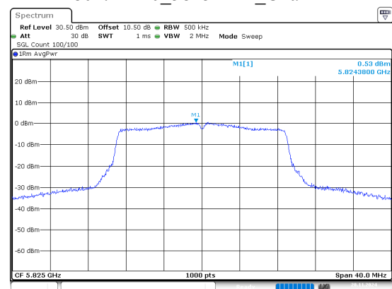
802.11n20_5825MHz_Chain 1
