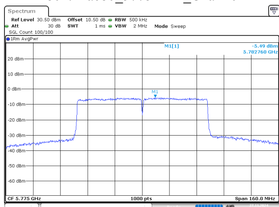
802.11ac80_5775MHz_Chain 0
