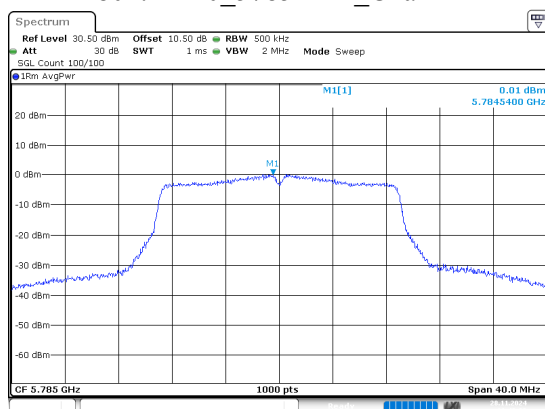
802.11n20_5785MHz_Chain 1
