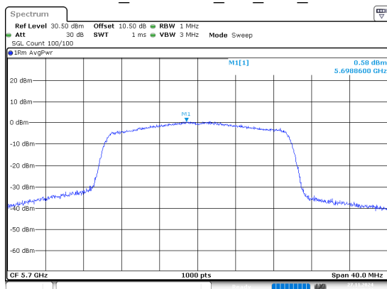
802.11ax20_5700MHz_RU_Full_Chain 0
