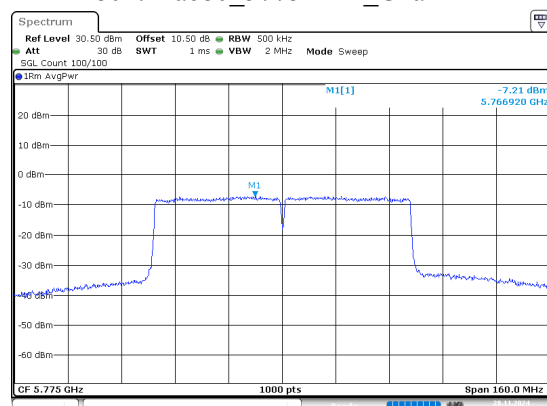
802.11ac80_5775MHz_Chain 1
