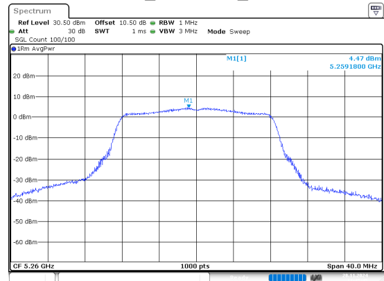
802.11a_5260MHz_Chain 1
