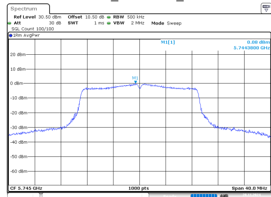
802.11n20_5745MHz_Chain 1
