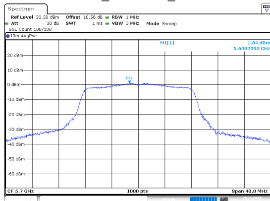
802.11a_5700MHz_Chain 1
