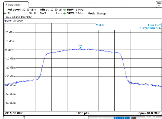
802.11ax20_5580MHz_RU_Full_Chain 0
