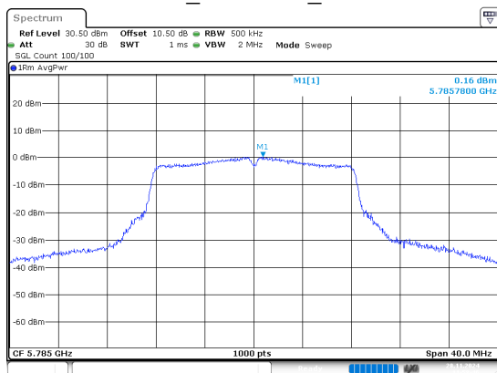
802.11a_5785MHz_Chain 1
