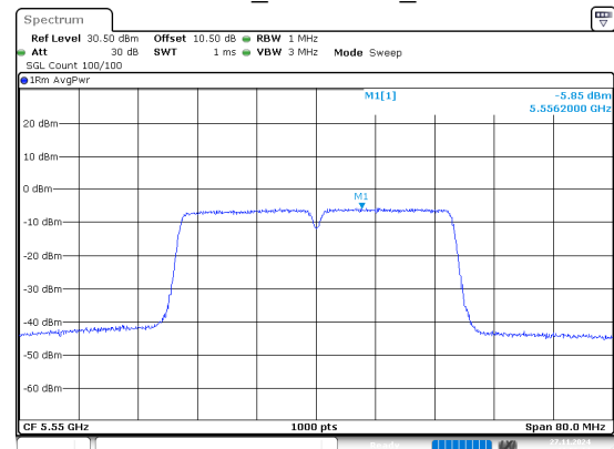
802.11n40_5550MHz_Chain 0
