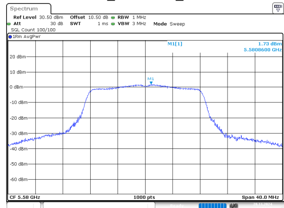
802.11a_5580MHz_Chain 1
