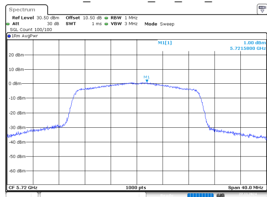
802.11ax20_5720MHz_RU_Full_Chain 0
