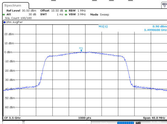
802.11ax20_5500MHz_RU_Full_Chain 1
