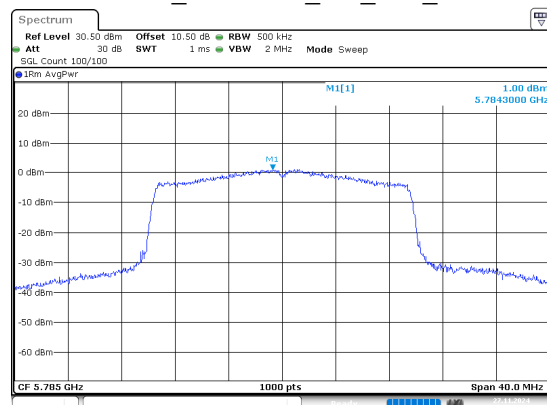
802.11ax20_5785MHz_RU_Full_Chain 0
