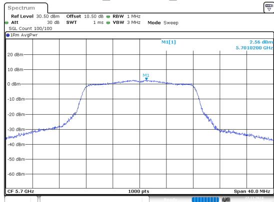
802.11a_5700MHz_Chain 0
