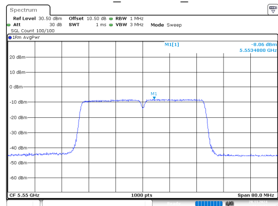
802.11n40_5550MHz_Chain 1
