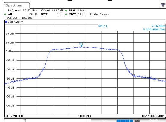
802.11n20_5280MHz_Chain 0
