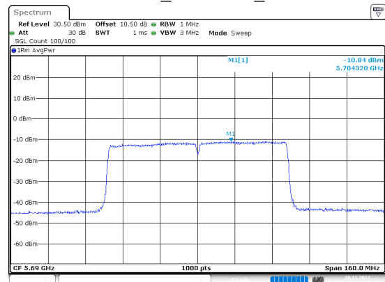
802.11ac80_5690MHz_Chain 1
