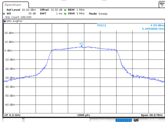
802.11a_5500MHz_Chain 0
