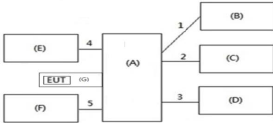
Test Setup Diagram - Conducted emission and Radiated emission below 1GHz
