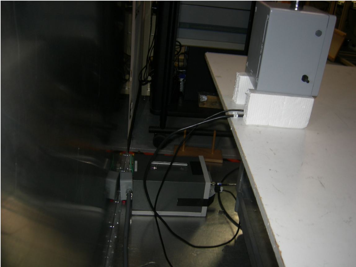
Figure 5: AC Power Line Conducted Emissions
