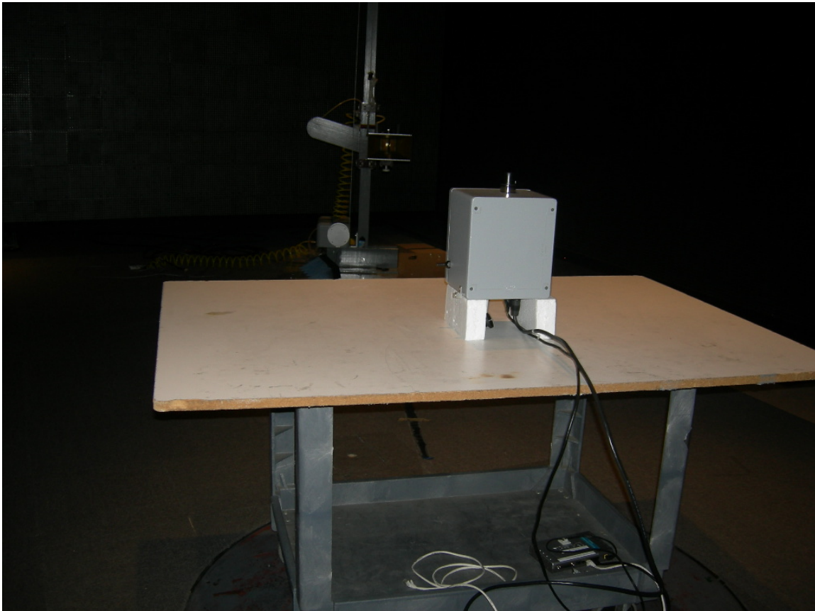
Figure 2: Radiated Emissions
