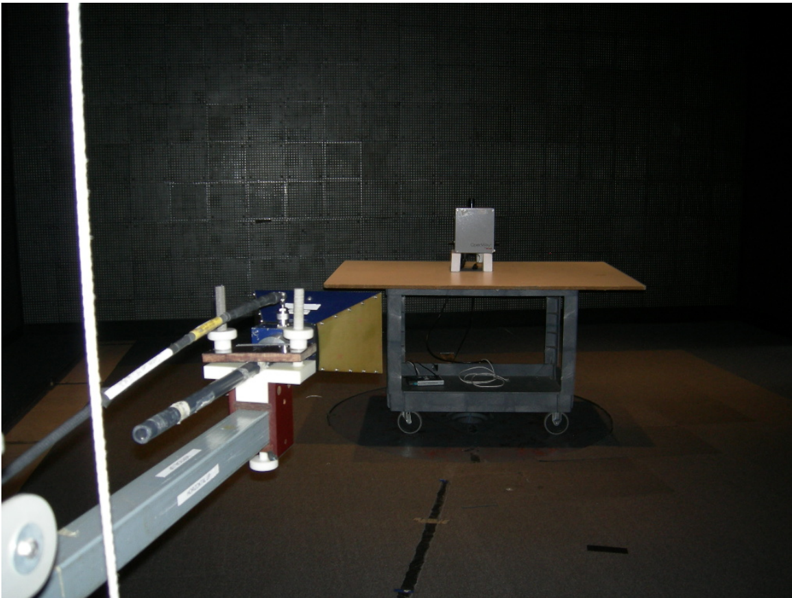
Figure 3: Radiated Emissions
