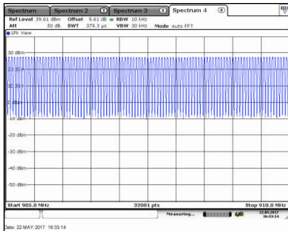
Figure 7.4.2.2-2: No. of Hop Channels – FSK – 10kbps
