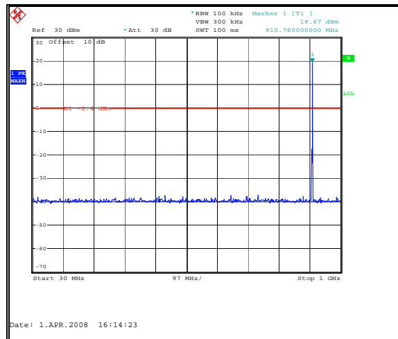
Figure 7.6.2-1 RF Conducted Spurious Emissions – Low Channel
