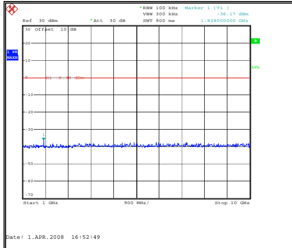
Figure 7.6.2-6 RF Conducted Spurious Emissions – High Channel
