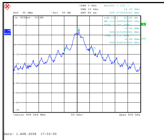
Figure 7.5.4-1: 20dB Bandwidth Low Channel
