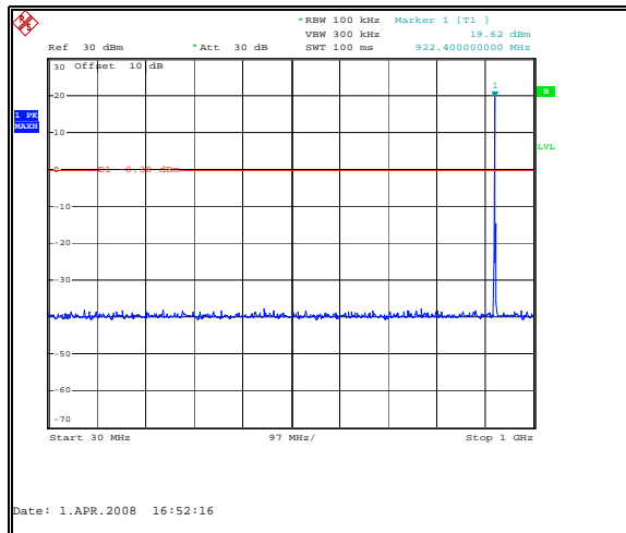
Figure 7.6.2-5 RF Conducted Spurious Emissions – High Channel
