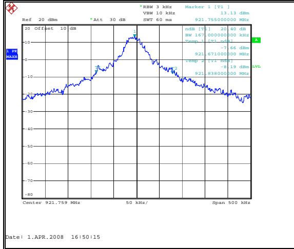
Figure 7.5.4-3: 20dB Bandwidth High Channel
