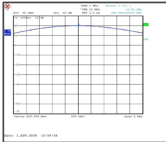
Figure 7.4-1: Output power – Low Channel
