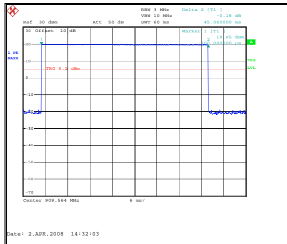
Figure 7.5.3-1: Channel Dwell Time
