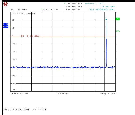
Figure 7.6.2-3 RF Conducted Spurious Emissions – Mid Channel
