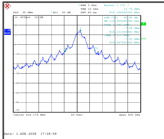
Figure 7.5.4-2: 20dB Bandwidth Mid Channel
