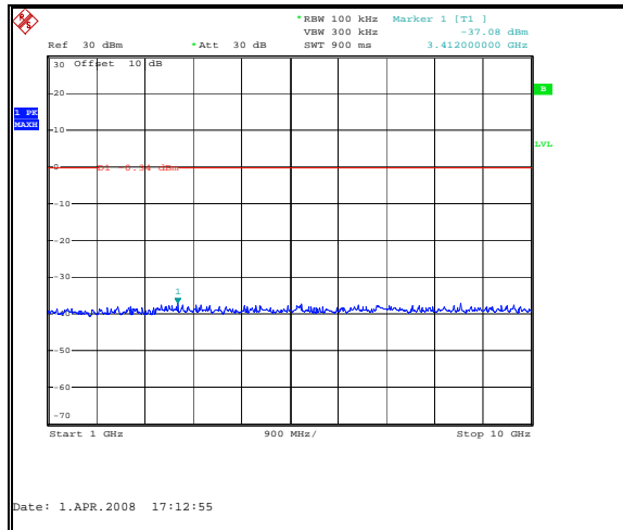
Figure 7.6.2-4 RF Conducted Spurious Emissions – Mid Channel
