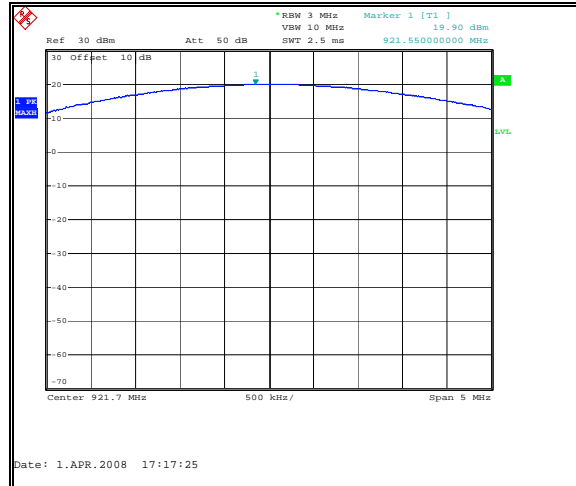
Figure 7.4-3: Output power – High Channel
