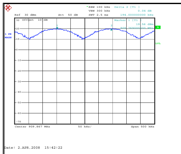
Figure 7.5.1-1: Carrier Frequency Separation
