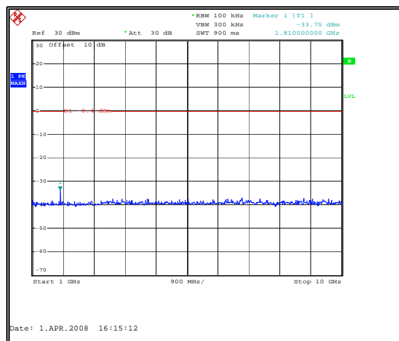
Figure 7.6.2-2 RF Conducted Spurious Emissions – Low Channel
