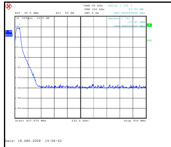
Figure 7.6.1-2: Upper Band-edge
