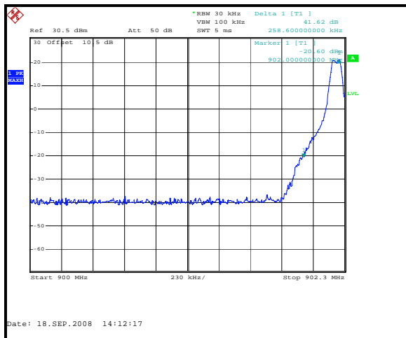
Figure 7.6.1-1: Lower Band-edge
