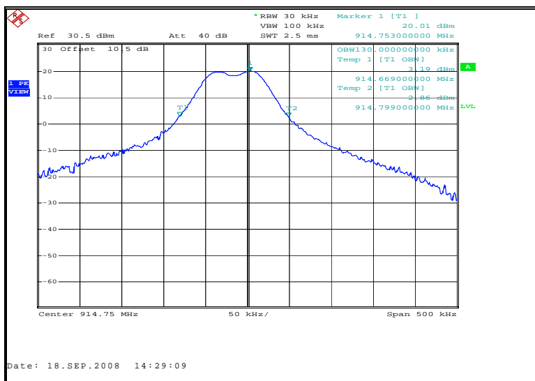
Figure 7.5.4-5: 99% Bandwidth Mid Channel
