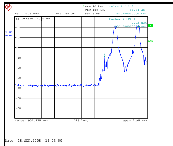
Figure 7.6.1-3: Lower Band-edge - Hopping
