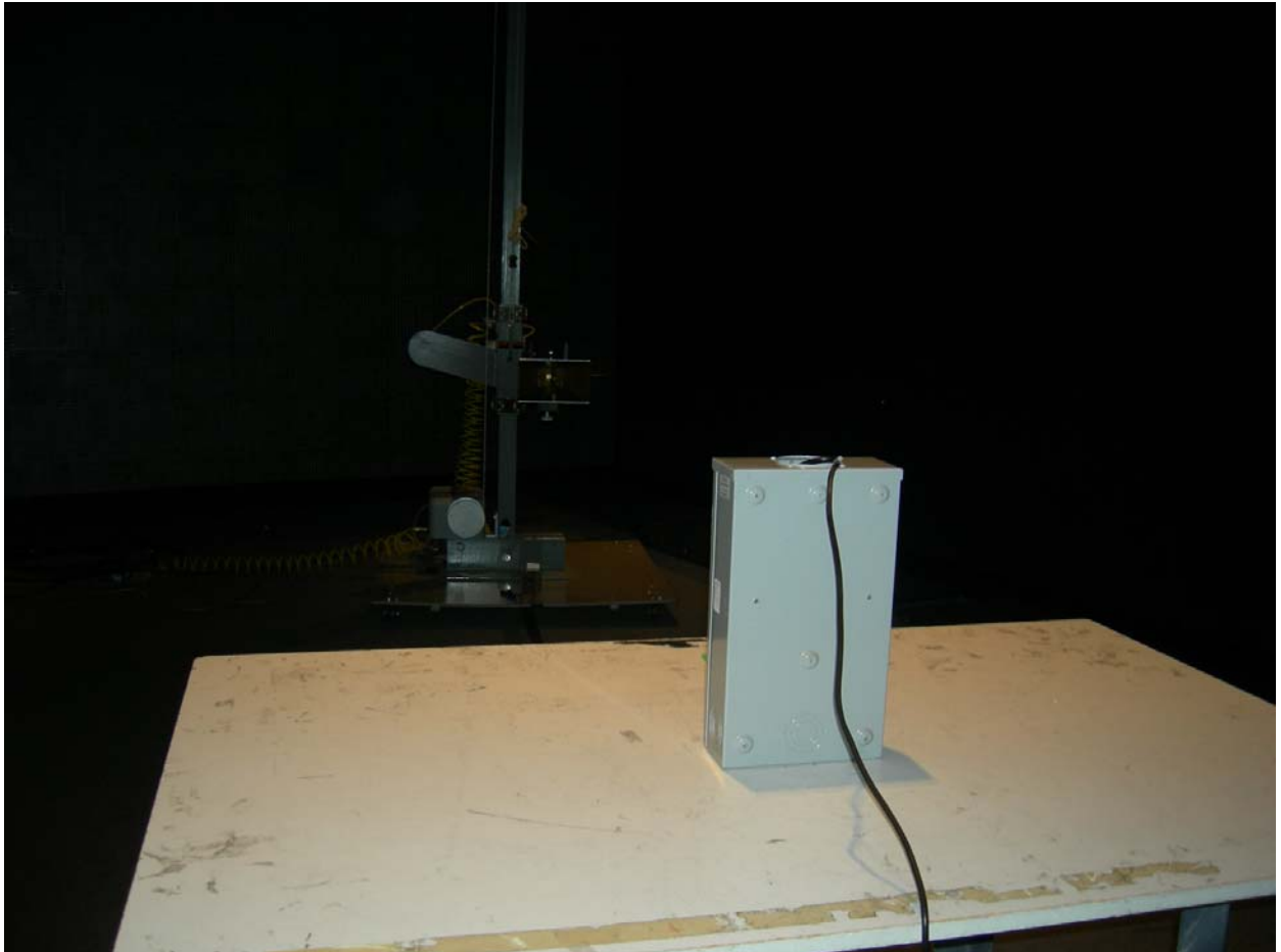
Figure 2: Radiated Emissions
