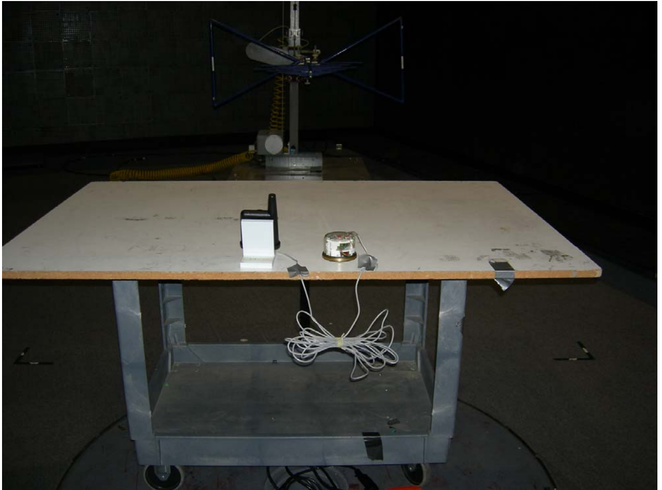
Figure 1: Test Setup Radiated Emissions - Unintentional
