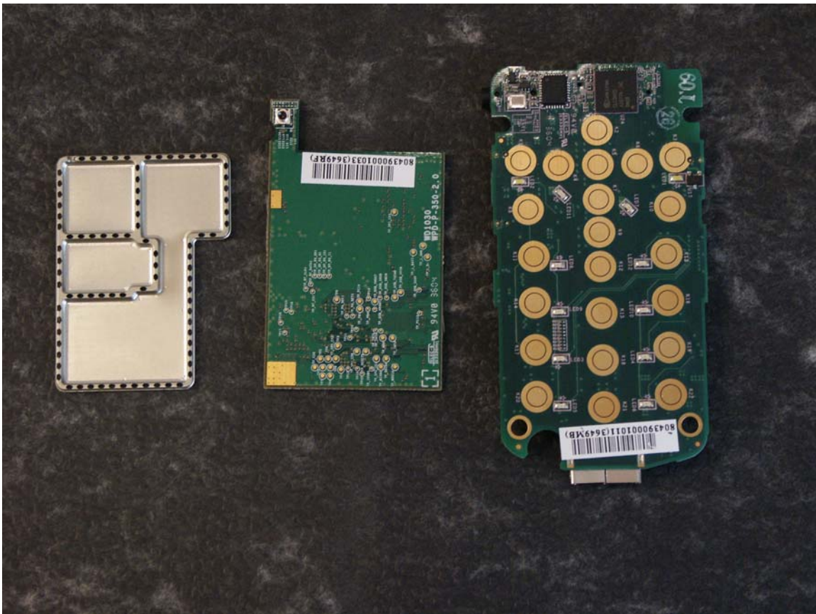
Photo 2. Back side view of radio PCB with shield removed (middle). Keypad board (right)
