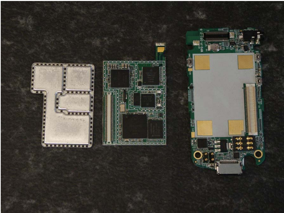
Photo 1. Front side view of radio PCB with shield removed (middle). Backside of Keypad board (right)
