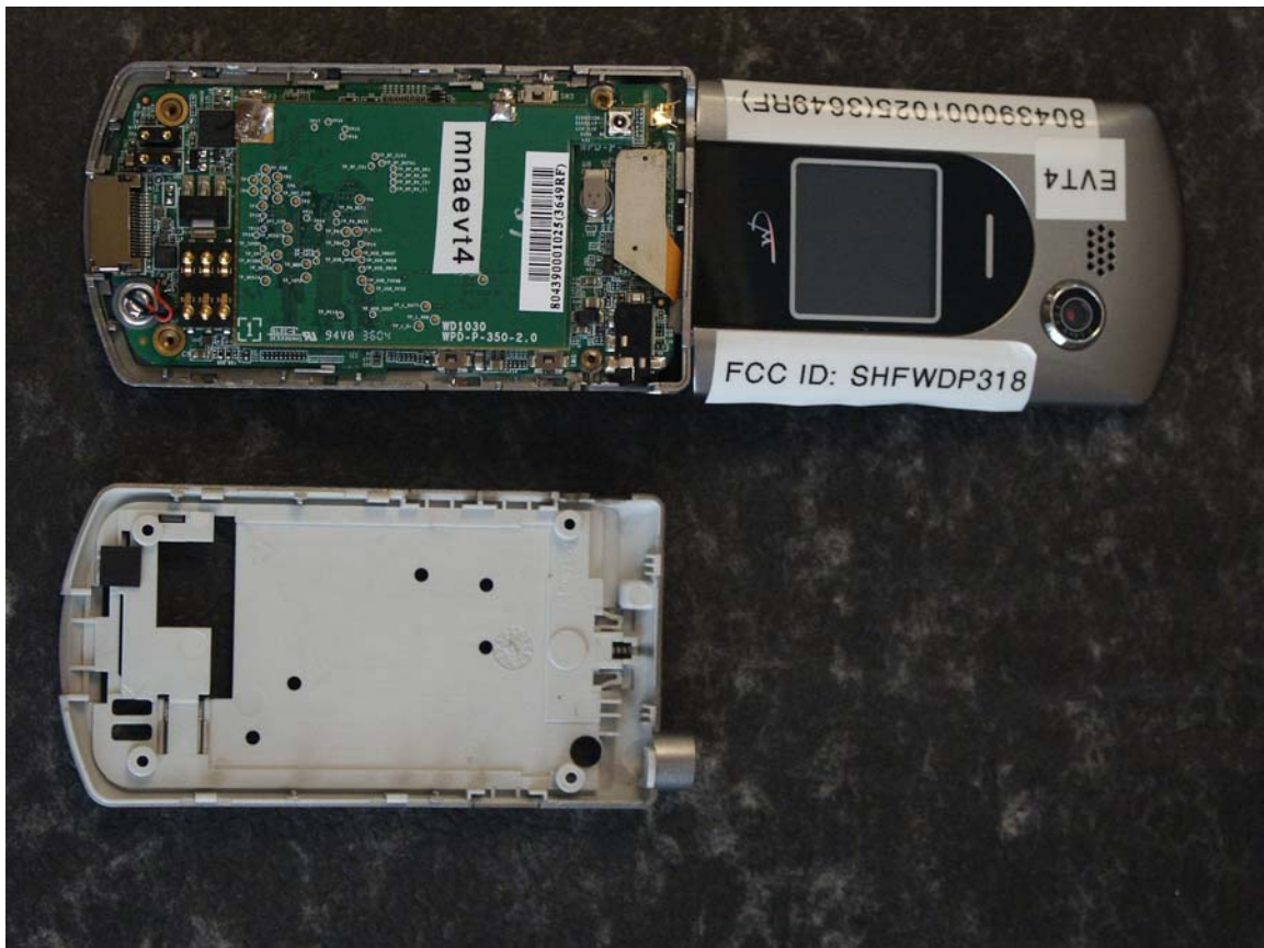
Photo 5. Radio board and Keypad board attached to internal and external Display Flexible board
