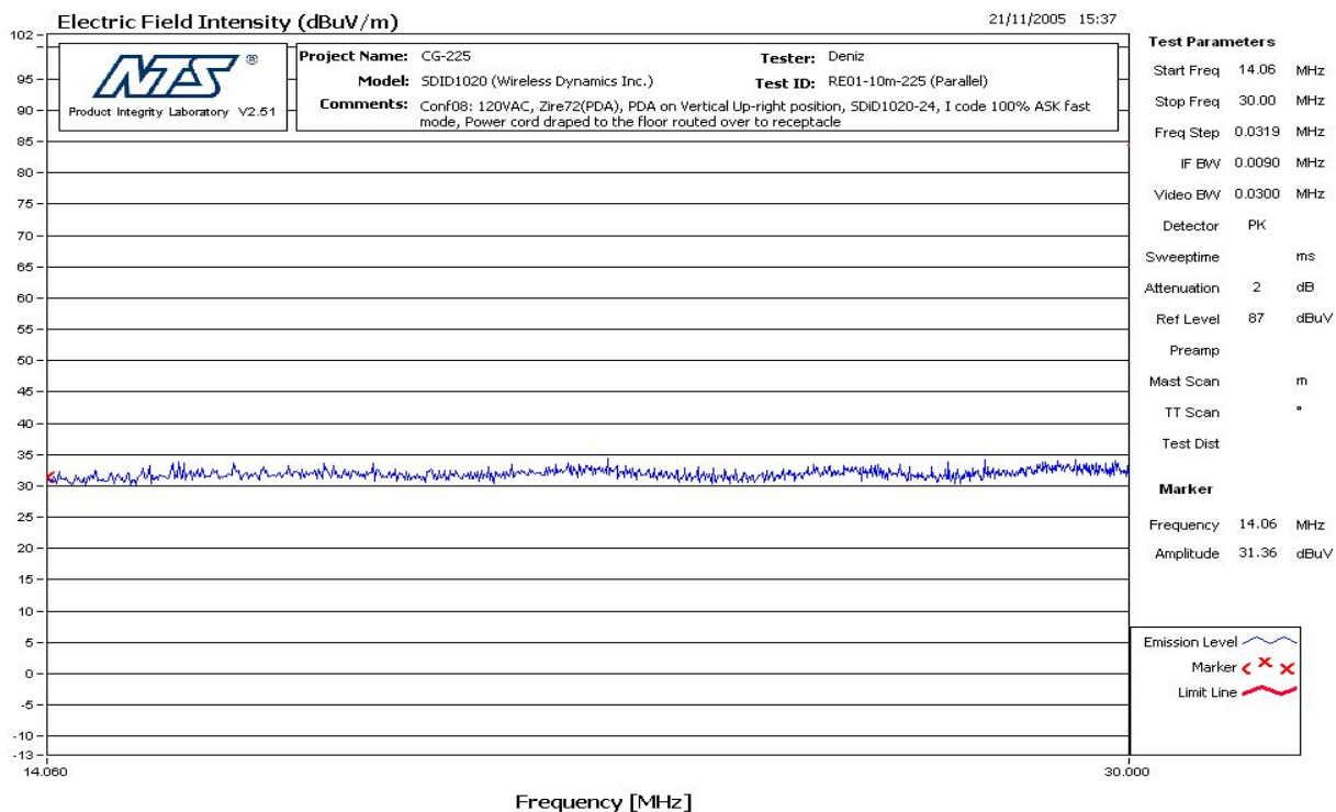
Figure 11 RE - Parallel – 14.06MHz – 30.0MHz
