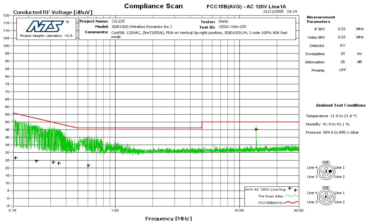
Figure 5 CE –Line A1 – 150 kHz – 30 MHz (Average Detector)
