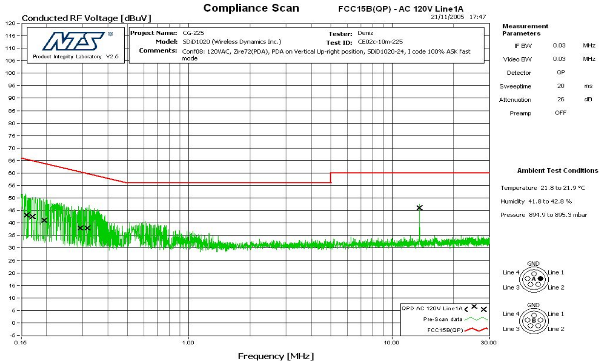
Figure 3 CE –Line A1 – 150 kHz – 30 MHz (QP Detector)
