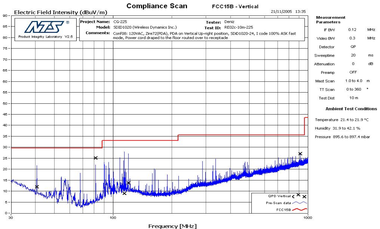
Figure 2 RE - Vertical – 30 MHz – 1 GHz
