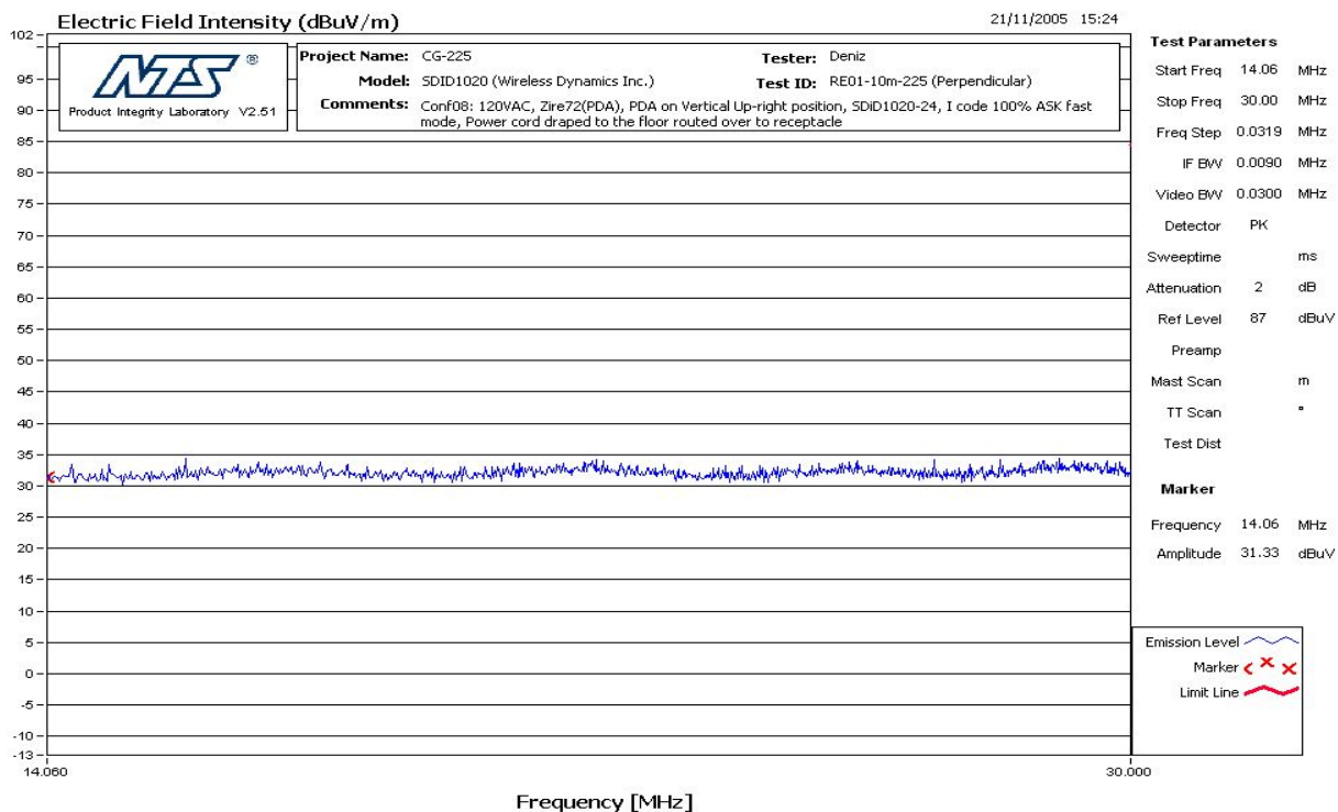
Figure 14 RE - Perpendicular – 14.06MHz – 30.0MHz
