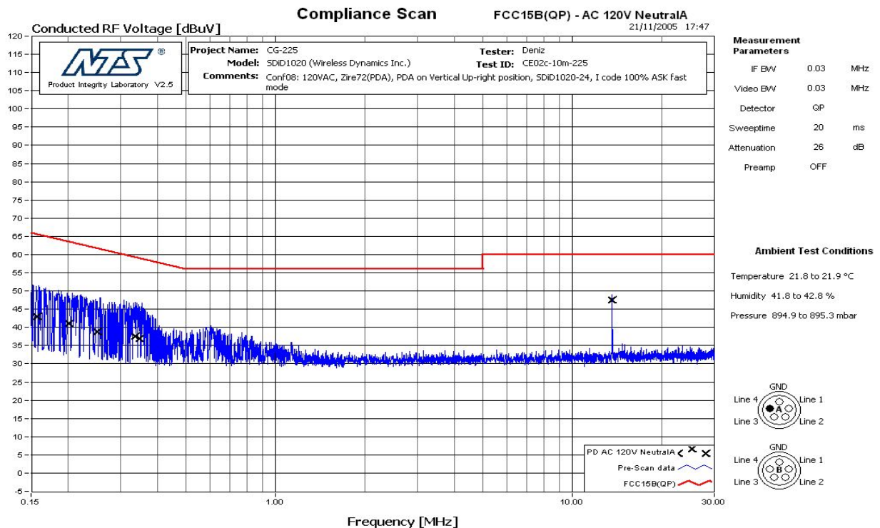
Figure 4 CE –Return A2 – 150 kHz – 30 MHz (QP Detector)
