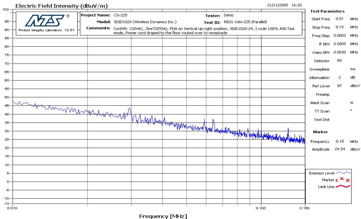
Figure 9 RE - Parallel – 9kHz – 150kHz
