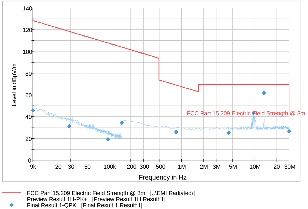
Discrete Rotation TUV 3m Radiated 9kHz to 30MHz..
