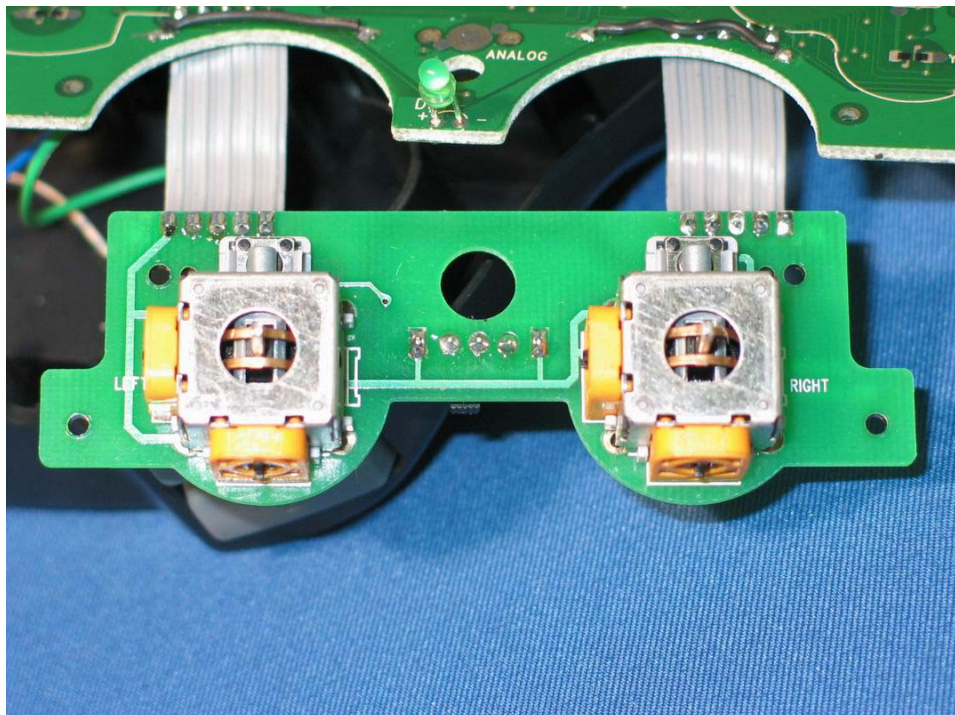
Internal Photo - 9
