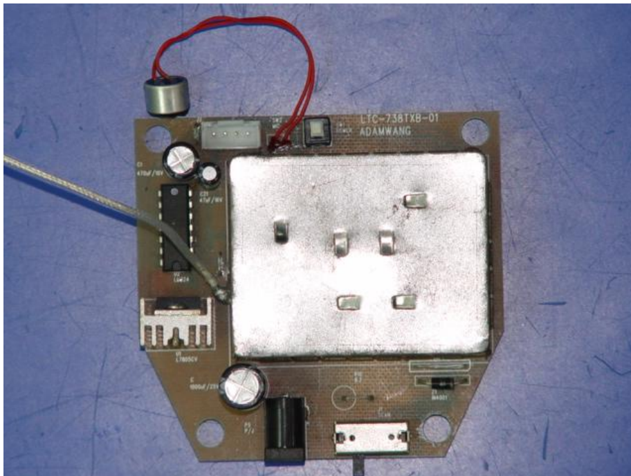
Photo6 PCB of Transmitter
