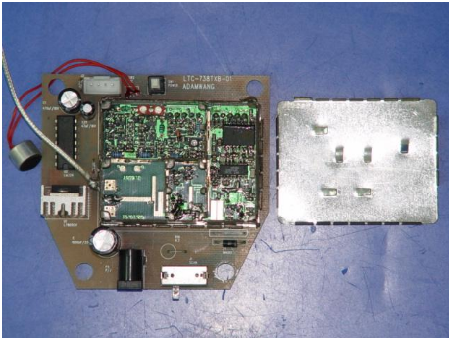
Photo8 PCB of Transmitter
