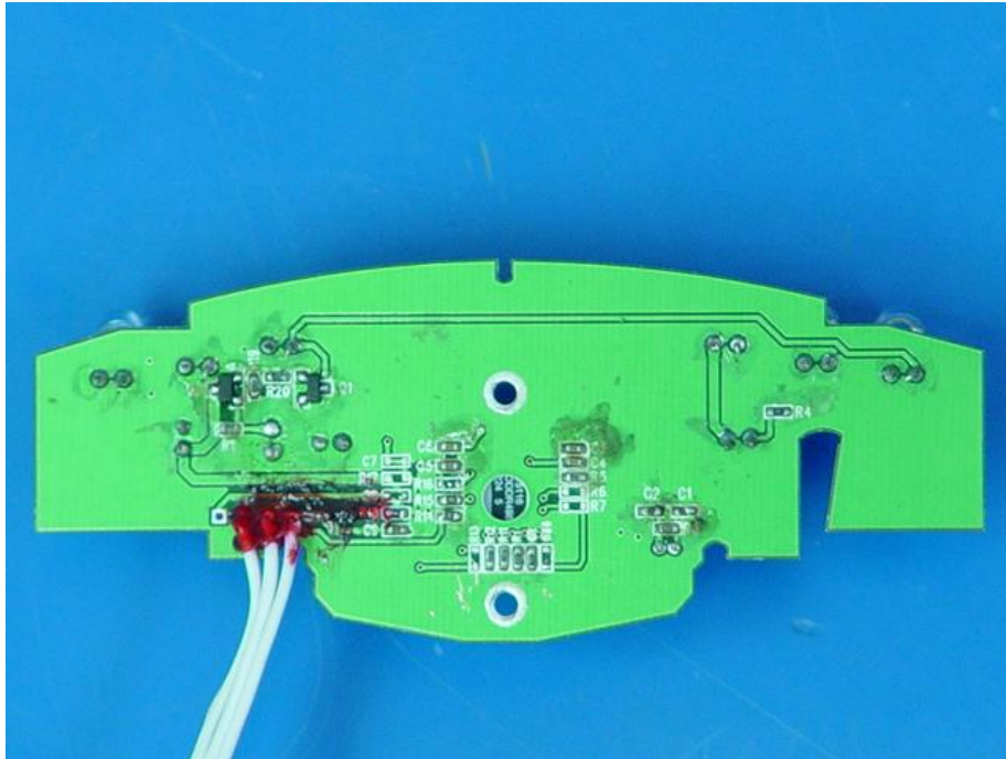
Photo5 PCB of Transmitter
