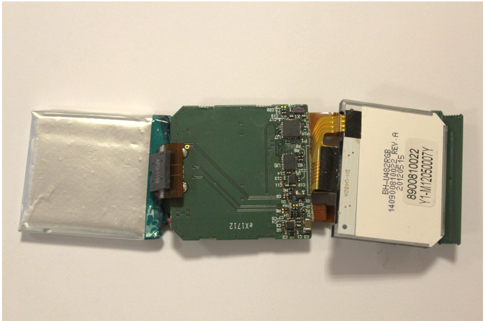
UBIWATCH21 device (FCC ID SEAWATCH21) – Internal view, host PCB+ LCD, front view
