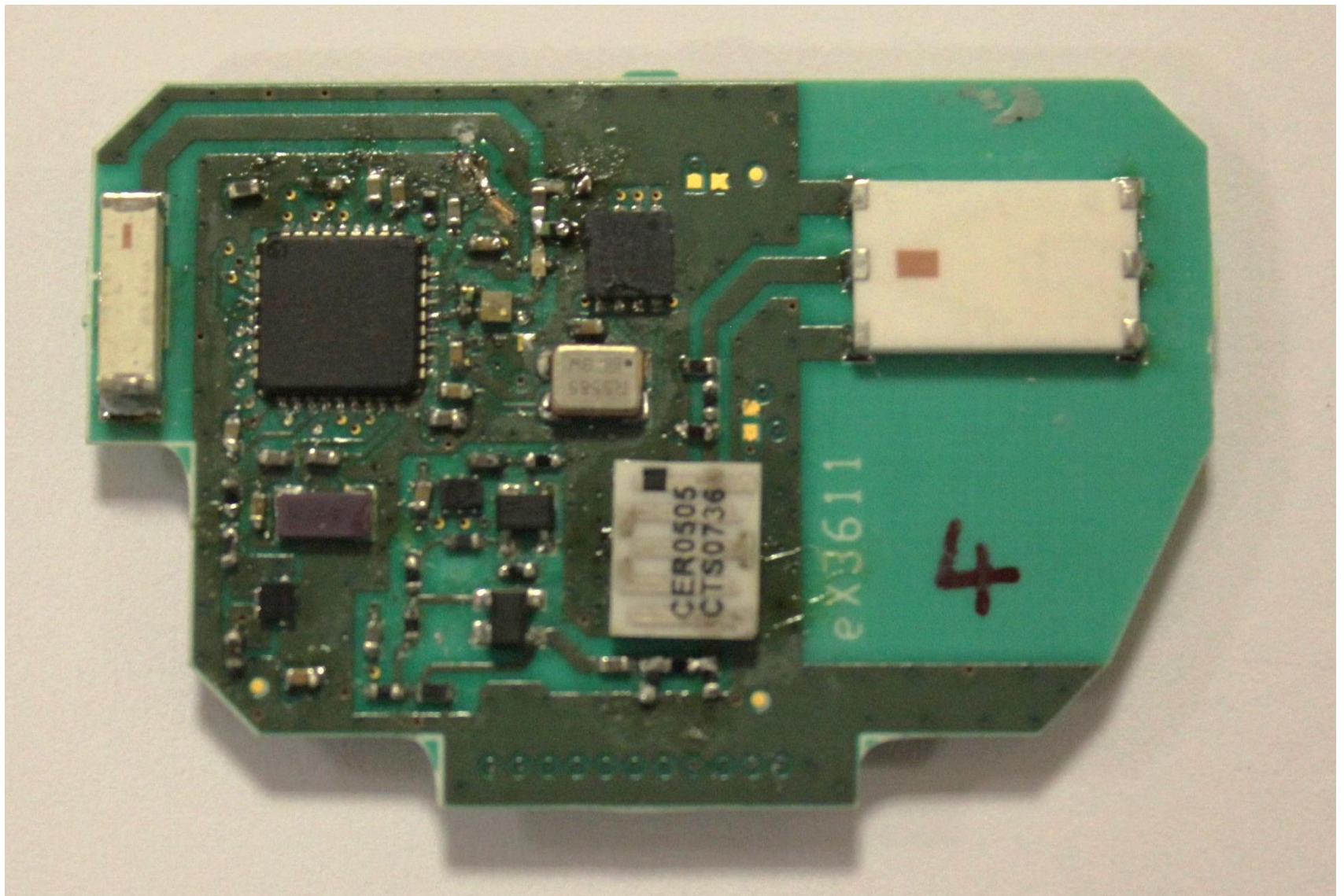
UBIWATCH21 device (FCC ID SEAWATCH21) – Internal view, UWB PCB, front view
