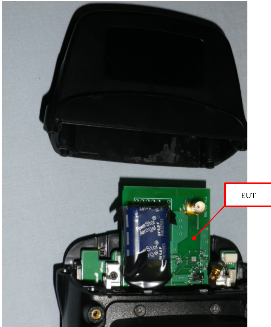
Figure 2: View of EUT with plastic cover removed Note: The Plastic cover is a prototype, and does not yet include the FCC/IC IDs. This circuit board has an SMA connector installed to make direct measurements To the 433MHz intentional radiator.
