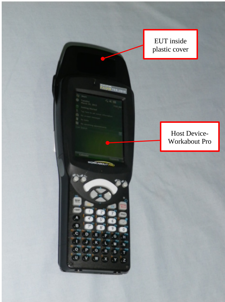
Figure 1: View of EUT on Workabout Pro Host hand held terminal.
