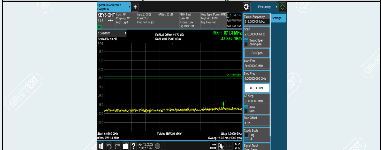
Band4-15MHz-QPSK-20175-1RB#0-Range1:30~1000MHz
