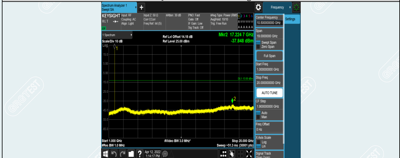
Band4-1.4MHz-16QAM-20393-1RB#0-Range2:1000~20000MHz
