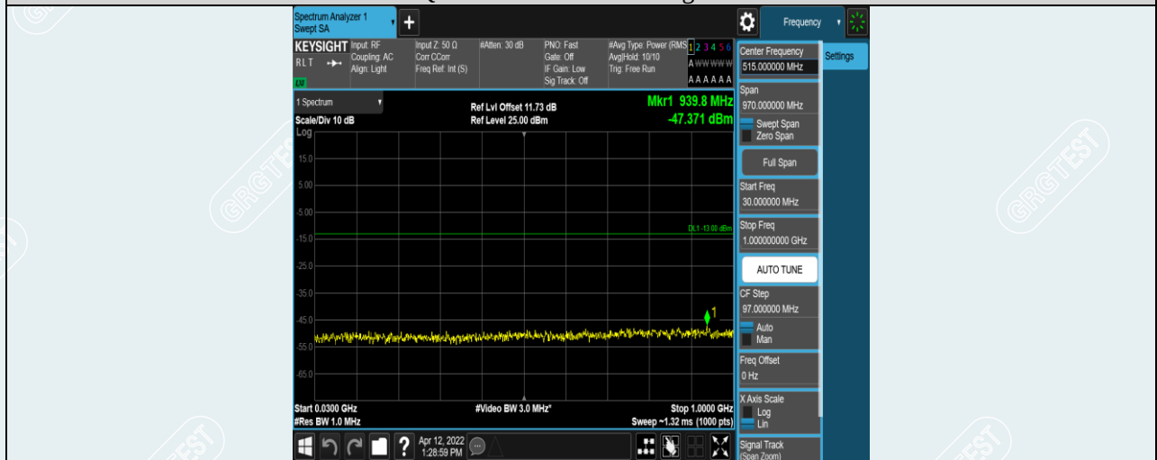
Band4-10MHz-QPSK-20350-1RB#0-Range1:30~1000MHz
