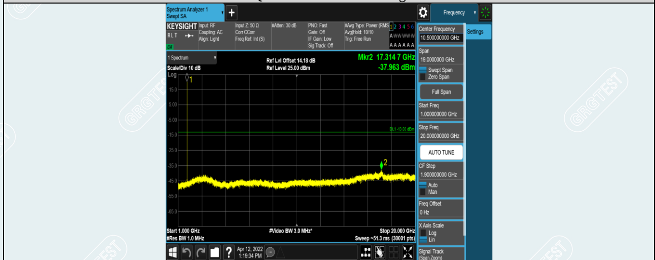
Band4-3MHz-16QAM-19965-1RB#0-Range2:1000~20000MHz
