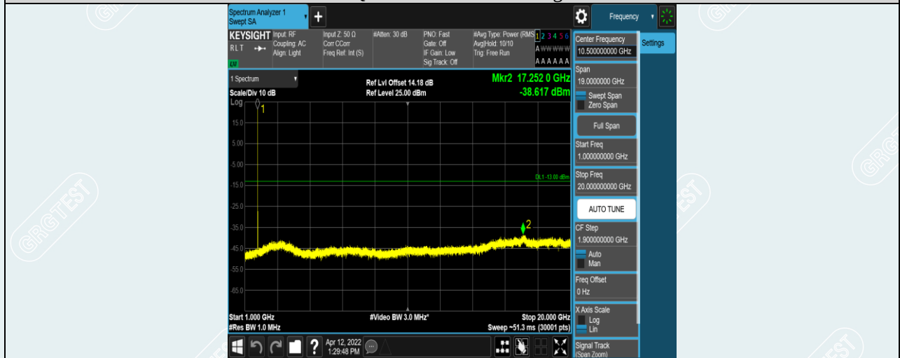
Band4-10MHz-16QAM-20350-1RB#0-Range2:1000~20000MHz
