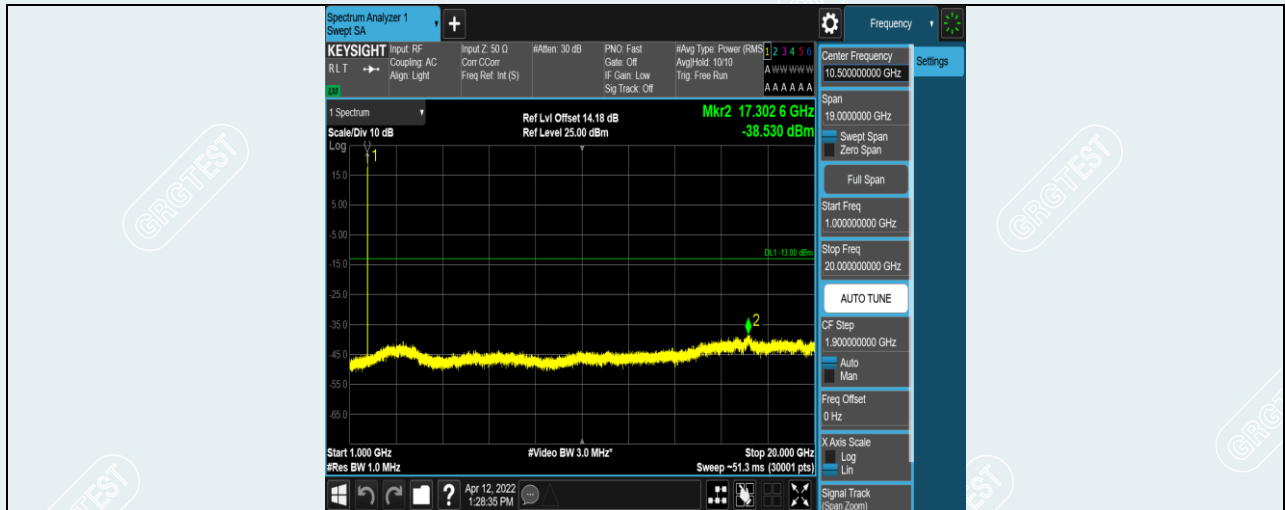
Band4-10MHz-16QAM-20175-1RB#0-Range2:1000~20000MHz
