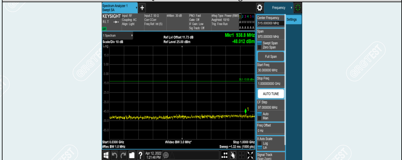
Band4-3MHz-16QAM-20385-1RB#0-Range1:30~1000MHz
