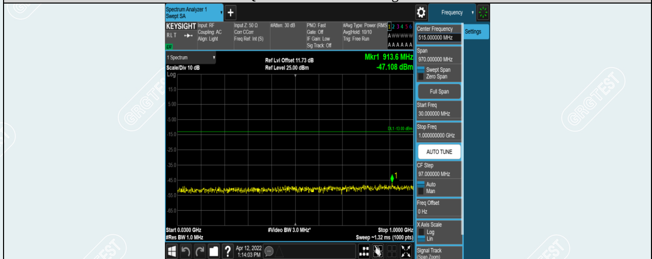
Band4-1.4MHz-16QAM-20393-1RB#0-Range1:30~1000MHz
