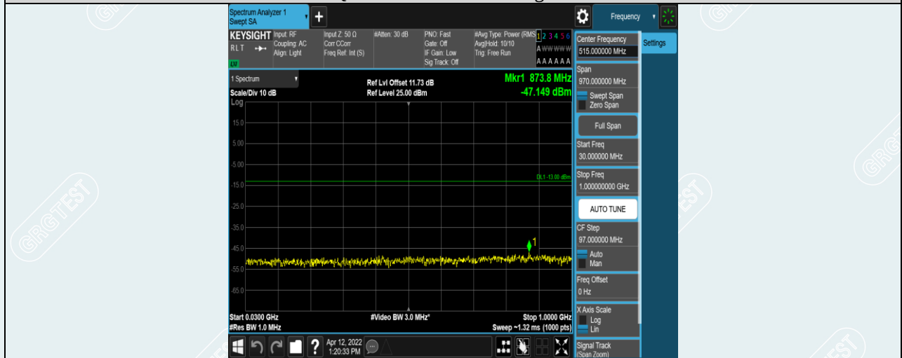
Band4-3MHz-16QAM-20175-1RB#0-Range1:30~1000MHz
