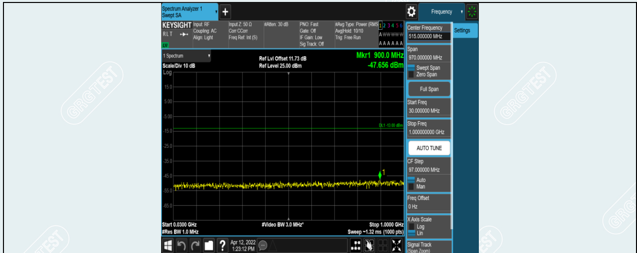
Band4-5MHz-16QAM-19975-1RB#0-Range1:30~1000MHz
