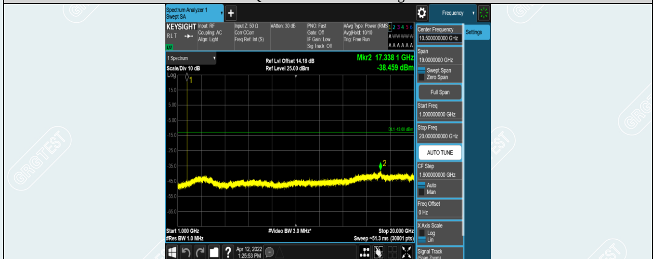
Band4-5MHz-16QAM-20375-1RB#0-Range2:1000~20000MHz
