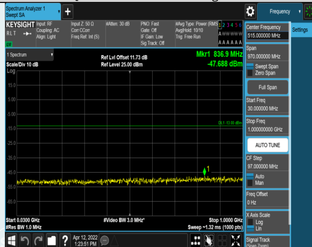
Band4-5MHz-QPSK-20175-1RB#0-Range1:30~1000MHz
