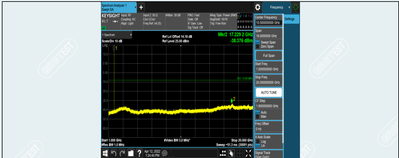
Band4-5MHz-16QAM-20175-1RB#0-Range2:1000~20000MHz
