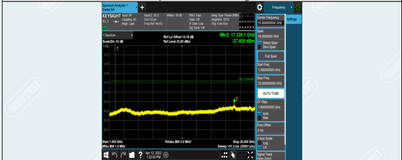
Band4-3MHz-16QAM-20385-1RB#0-Range2:1000~20000MHz
