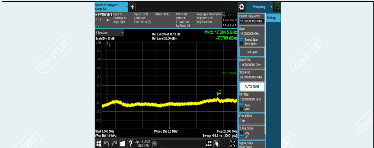
Band4-15MHz-QPSK-20175-1RB#0-Range2:1000~20000MHz
