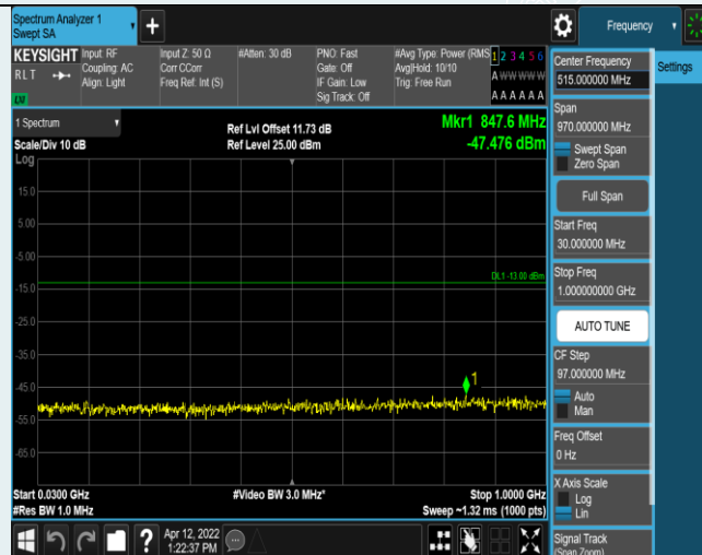
Band4-5MHz-QPSK-19975-1RB#0-Range1:30~1000MHz
