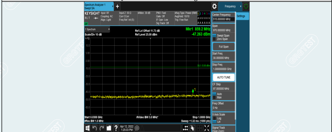
Band4-5MHz-QPSK-20375-1RB#0-Range1:30~1000MHz
