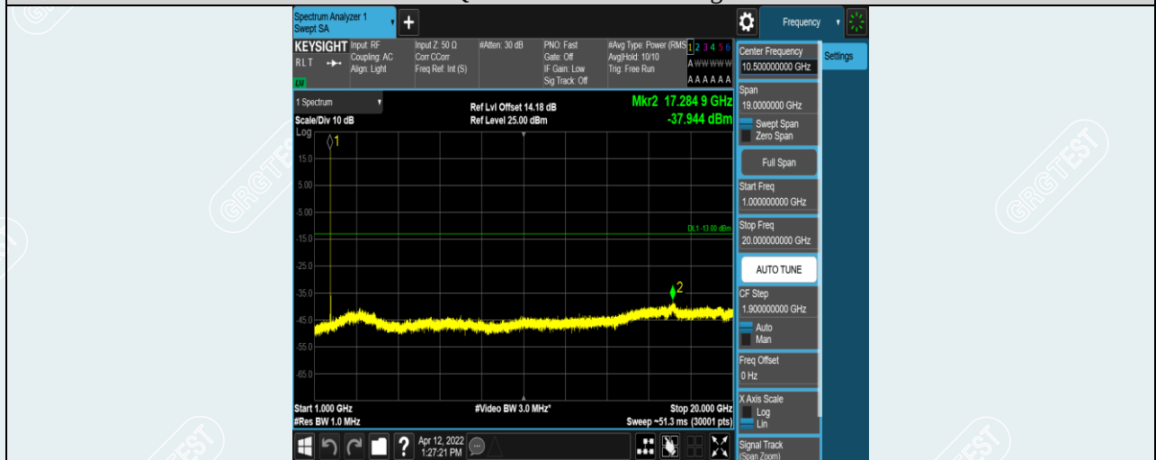
Band4-10MHz-16QAM-20000-1RB#0-Range2:1000~20000MHz
