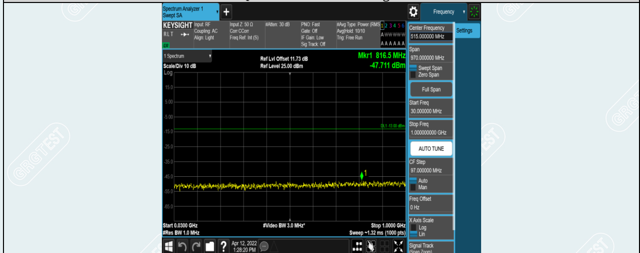
Band4-10MHz-16QAM-20175-1RB#0-Range1:30~1000MHz
