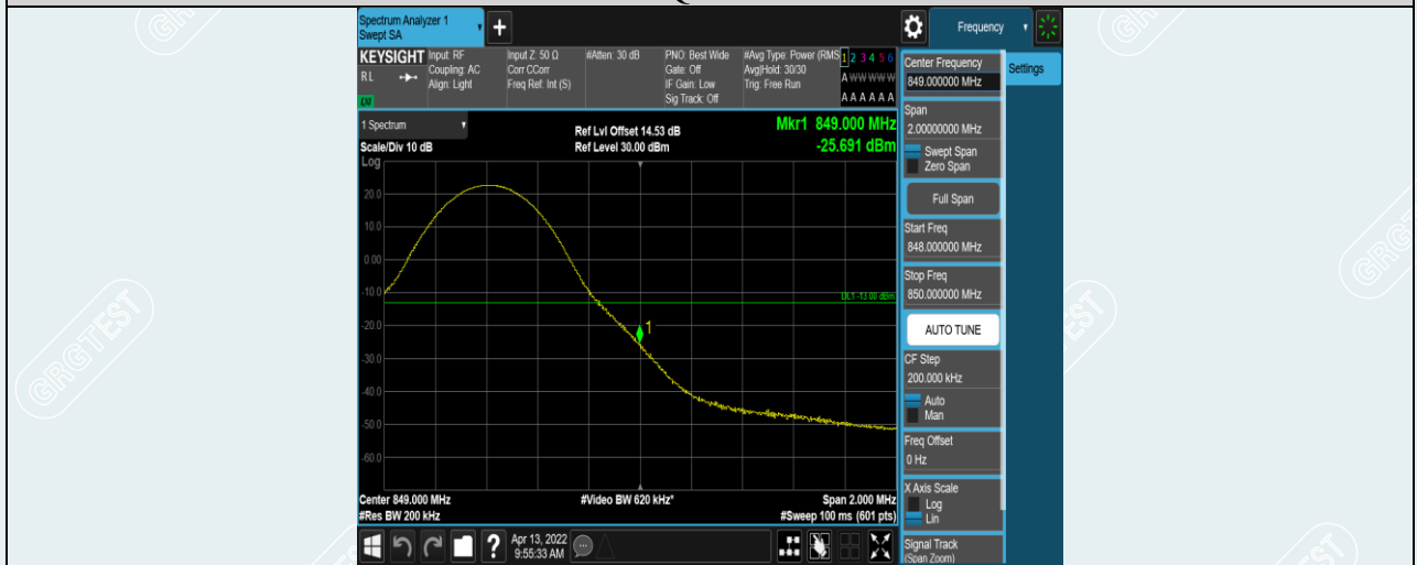
Band5-10MHz-QPSK-20600-1RB#49
