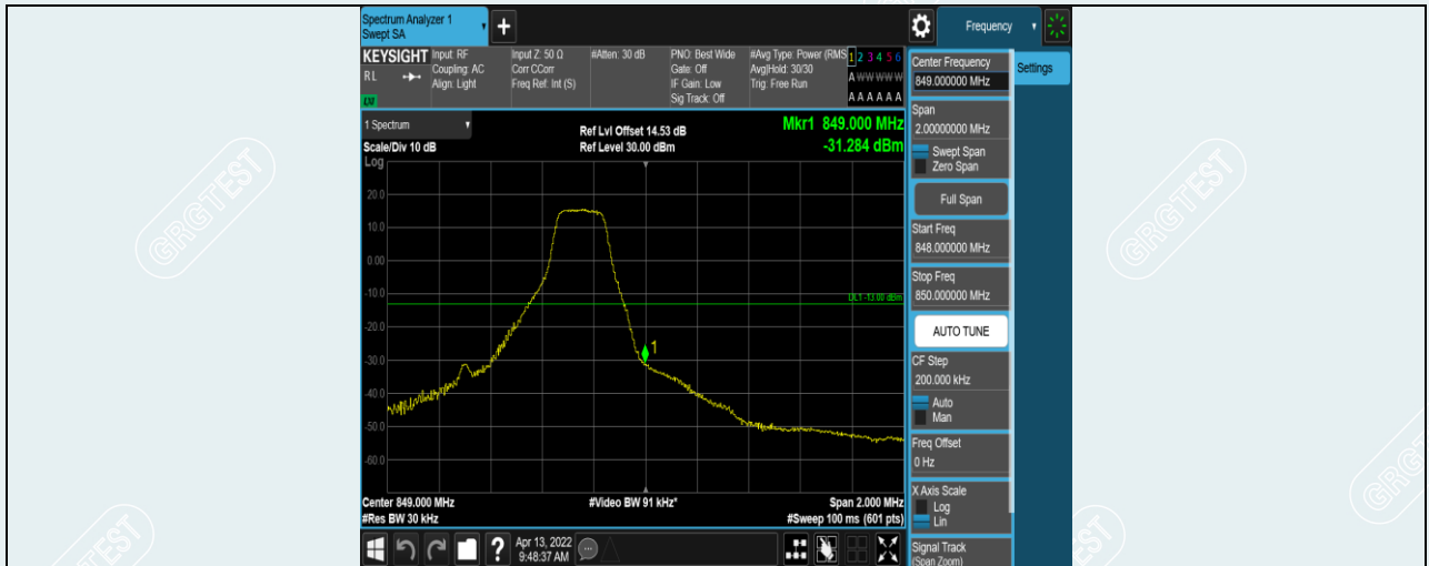
Band5-1.4MHz-16QAM-20643-1RB#5
