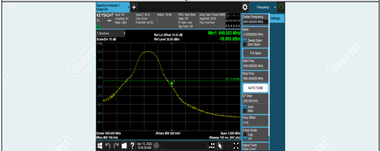
Band5-5MHz-16QAM-20625-1RB#24
