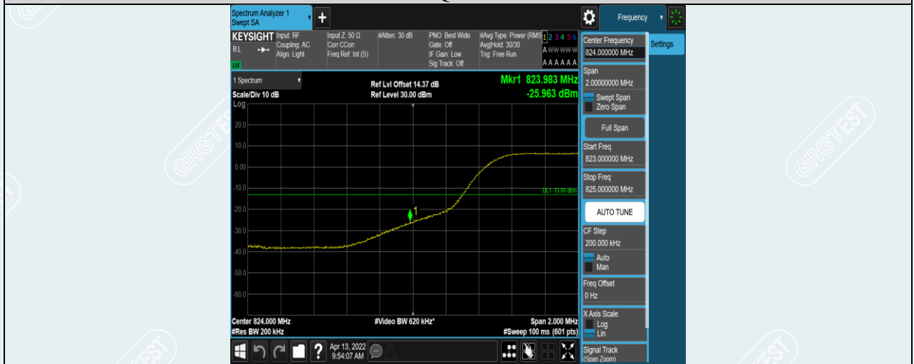
Band5-10MHz-QPSK-20450-50RB#0
