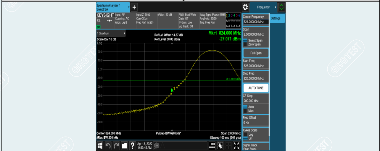
Band5-10MHz-16QAM-20450-1RB#0
