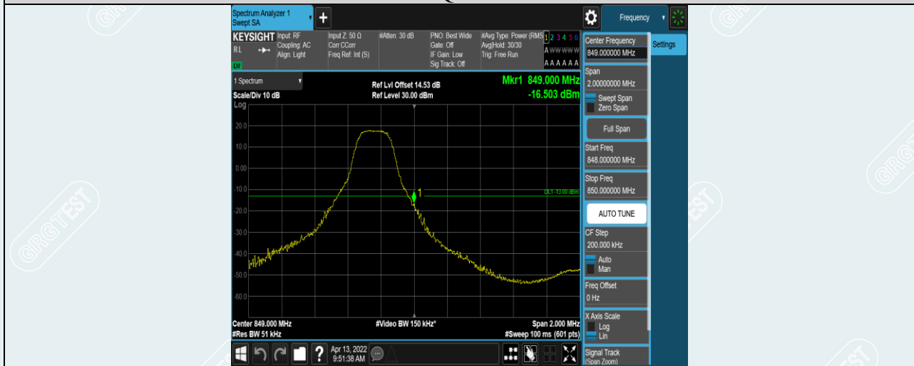
Band5-3MHz-16QAM-20635-1RB#14
