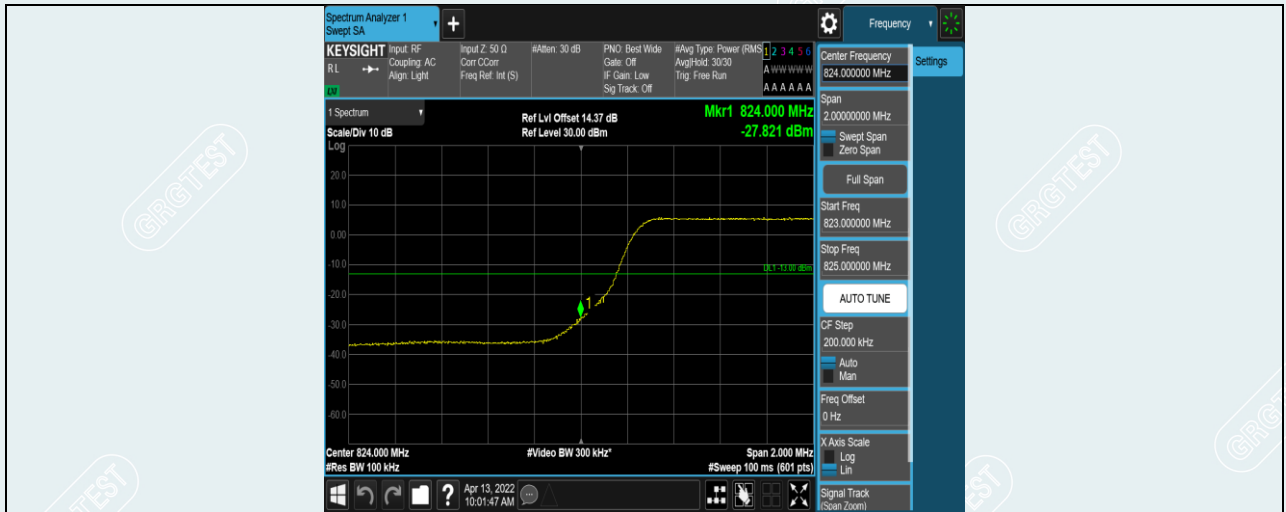
Band5-5MHz-16QAM-20425-25RB#0
