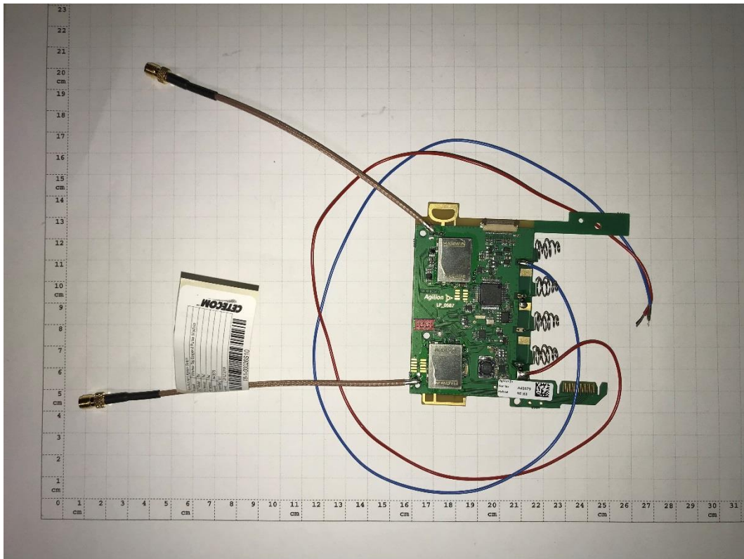
Photograph 8: EUT B, top view
