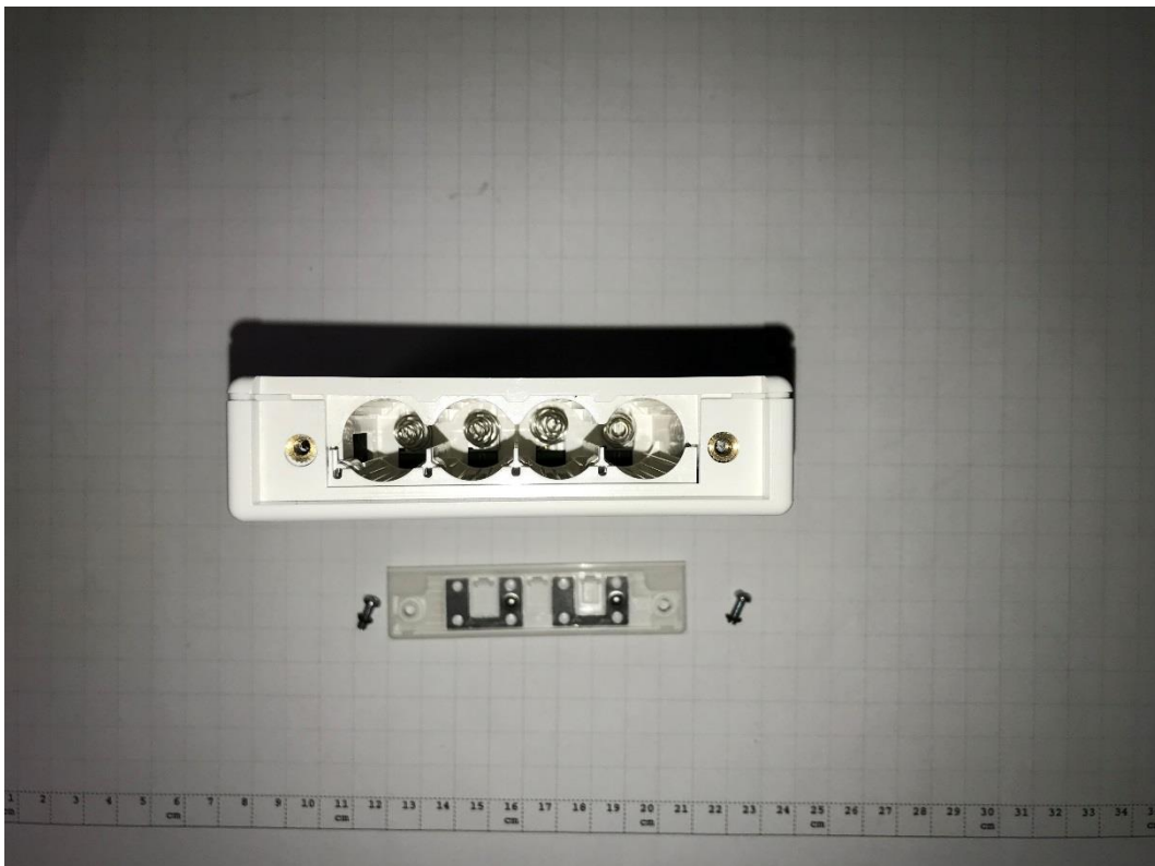
Photograph 6: EUT A, left side, cover open
