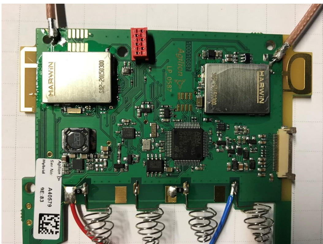
Photograph 2: EUT B, front close view, right- UWB antenna, left- 2,4 GHz antenna
